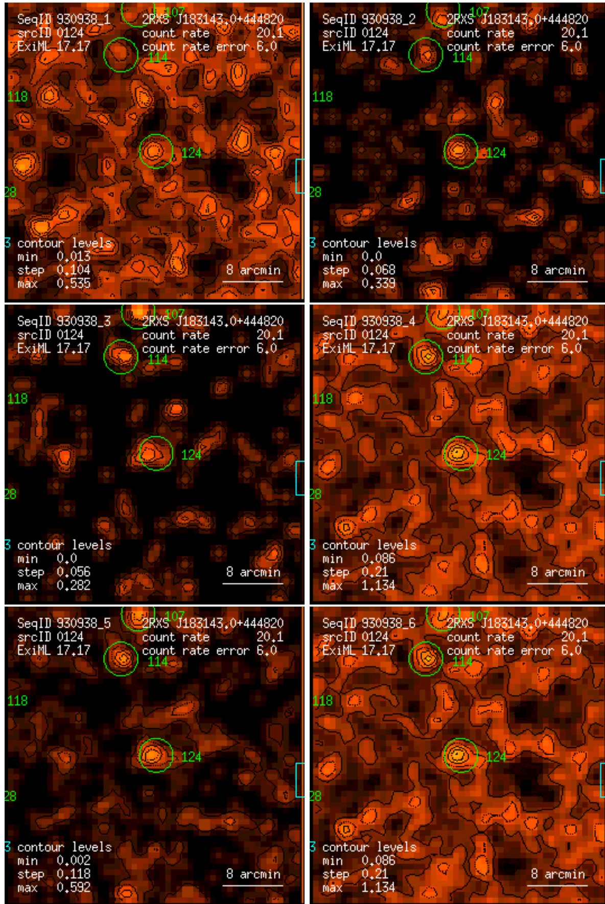
Figure 124: RASS 930938: detection 0124: band rate images, Gaussian filter: (1) PSPC channels 11 – 41, (2) 52 – 90, (3) 91 – 201, (4) 11 – 235, (5) 52 – 201, (6) 11 – 201. Broad band rates in counts/ks. Band rate contour levels in counts/ks/arcmin 2 .
