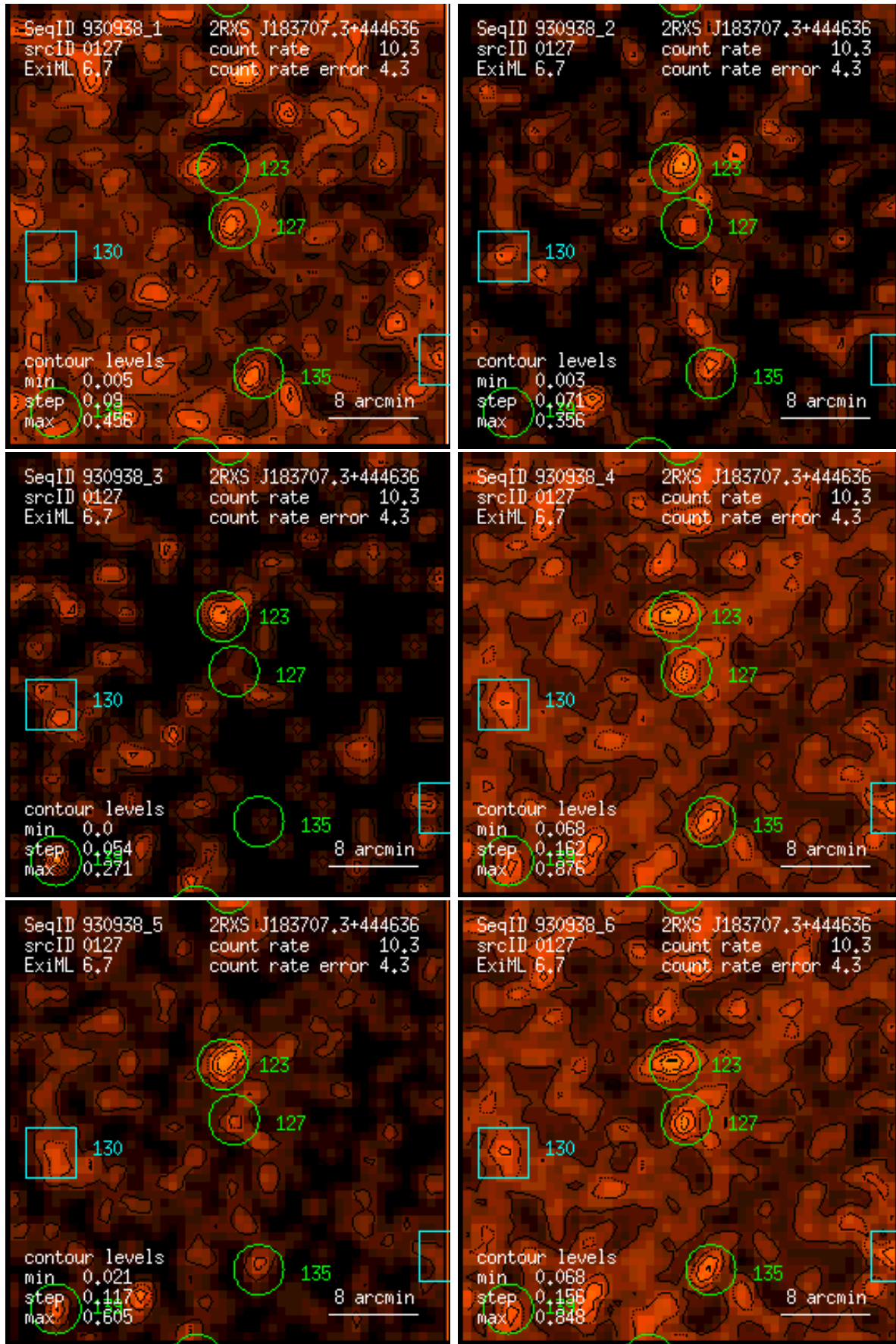
Figure 127: RASS 930938: detection 0127: band rate images, Gaussian filter: (1) PSPC channels 11 – 41, (2) 52 – 90, (3) 91 – 201, (4) 11 – 235, (5) 52 – 201, (6) 11 – 201. Broad band rates in counts/ks. Band rate contour levels in counts/ks/arcmin 2 .
