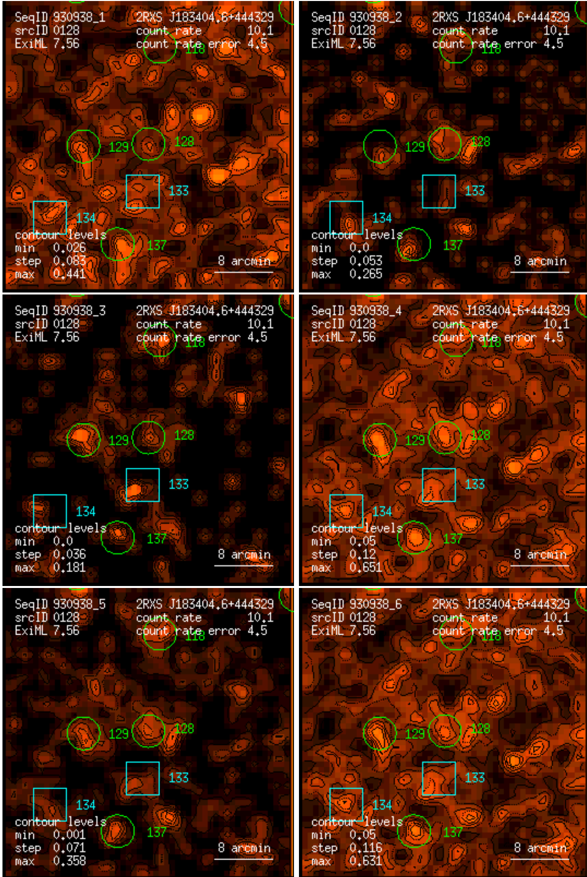
Figure 128: RASS 930938: detection 0128: band rate images, Gaussian filter: (1) PSPC channels 11 – 41, (2) 52 – 90, (3) 91 – 201, (4) 11 – 235, (5) 52 – 201, (6) 11 – 201. Broad band rates in counts/ks. Band rate contour levels in counts/ks/arcmin 2 .
