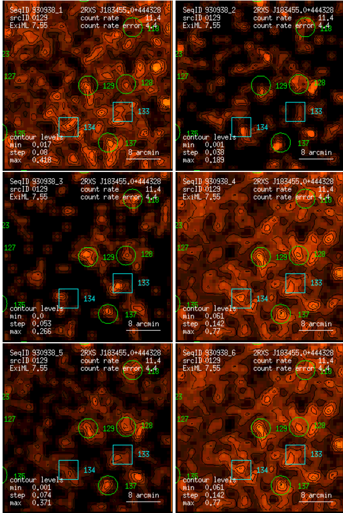
Figure 129: RASS 930938: detection 0129: band rate images, Gaussian filter: (1) PSPC channels 11 – 41, (2) 52 – 90, (3) 91 – 201, (4) 11 – 235, (5) 52 – 201, (6) 11 – 201. Broad band rates in counts/ks. Band rate contour levels in counts/ks/arcmin 2 .
