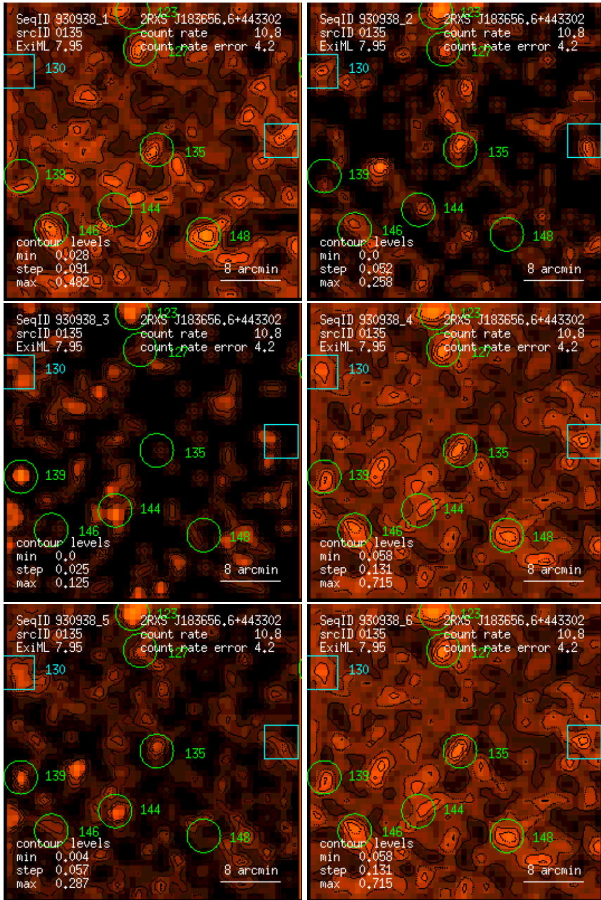
Figure 135: RASS 930938: detection 0135: band rate images, Gaussian filter: (1) PSPC channels 11 – 41, (2) 52 – 90, (3) 91 – 201, (4) 11 – 235, (5) 52 – 201, (6) 11 – 201. Broad band rates in counts/ks. Band rate contour levels in counts/ks/arcmin 2 .
