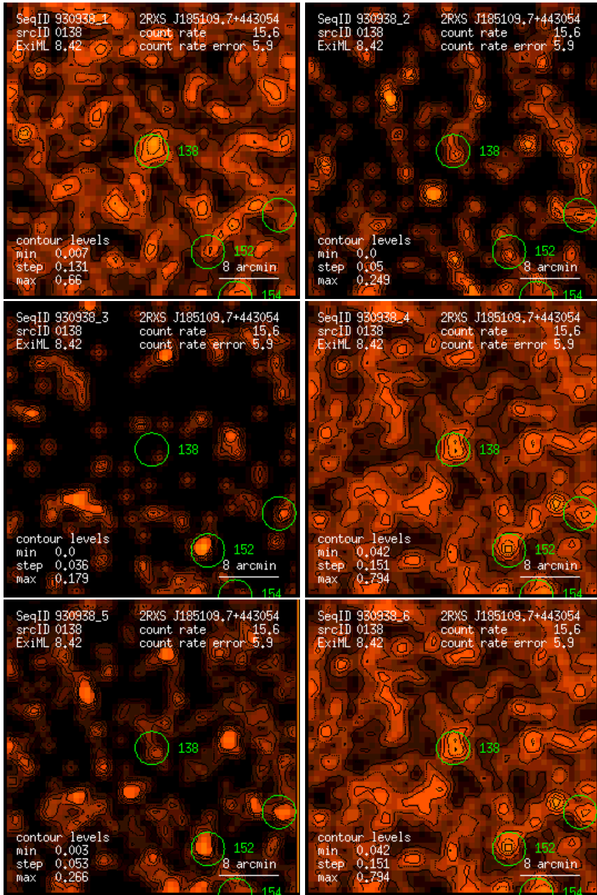
Figure 138: RASS 930938: detection 0138: band rate images, Gaussian filter: (1) PSPC channels 11 – 41, (2) 52 – 90, (3) 91 – 201, (4) 11 – 235, (5) 52 – 201, (6) 11 – 201. Broad band rates in counts/ks. Band rate contour levels in counts/ks/arcmin 2 .
