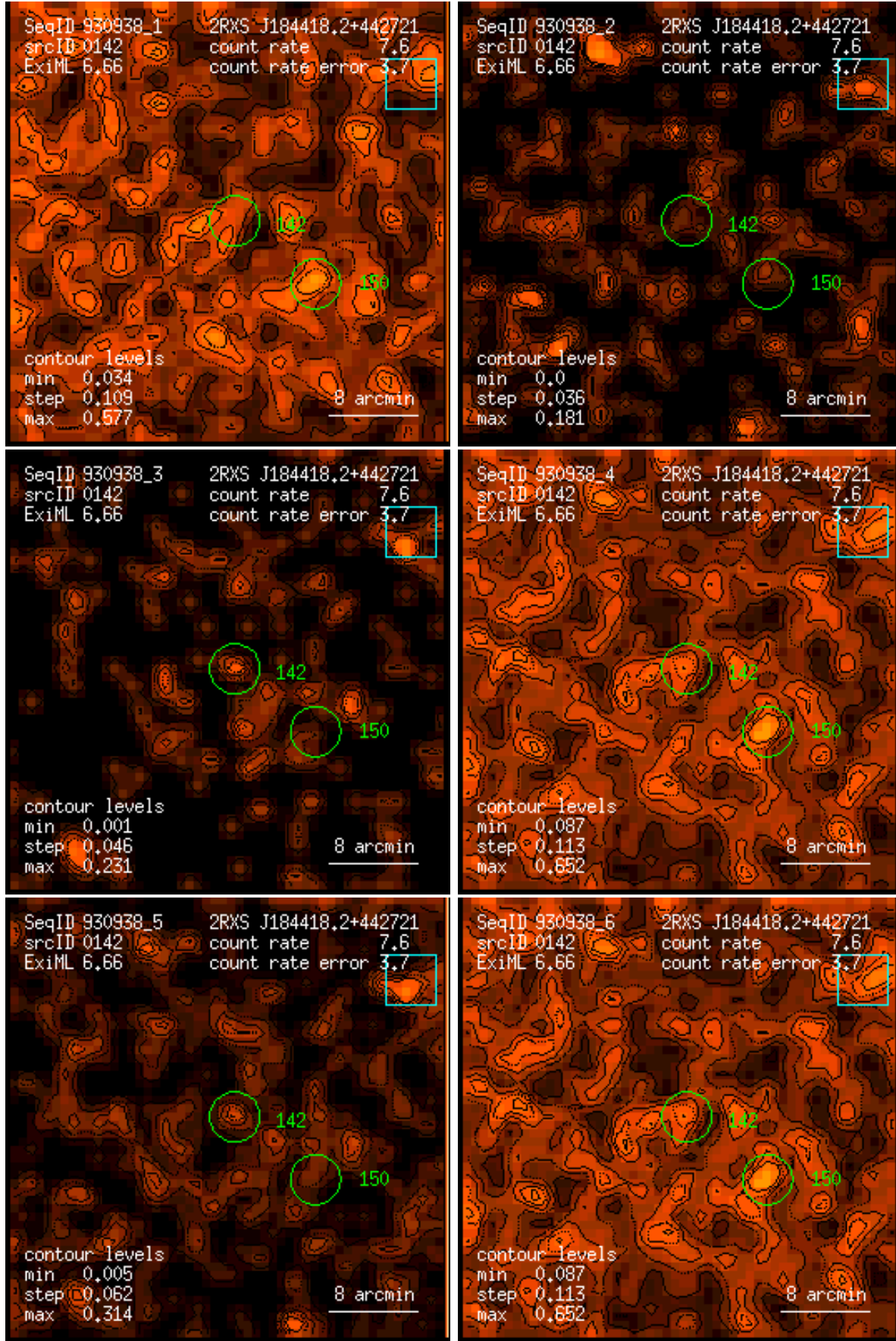
Figure 142: RASS 930938: detection 0142: band rate images, Gaussian filter: (1) PSPC channels 11 – 41, (2) 52 – 90, (3) 91 – 201, (4) 11 – 235, (5) 52 – 201, (6) 11 – 201. Broad band rates in counts/ks. Band rate contour levels in counts/ks/arcmin 2 .
