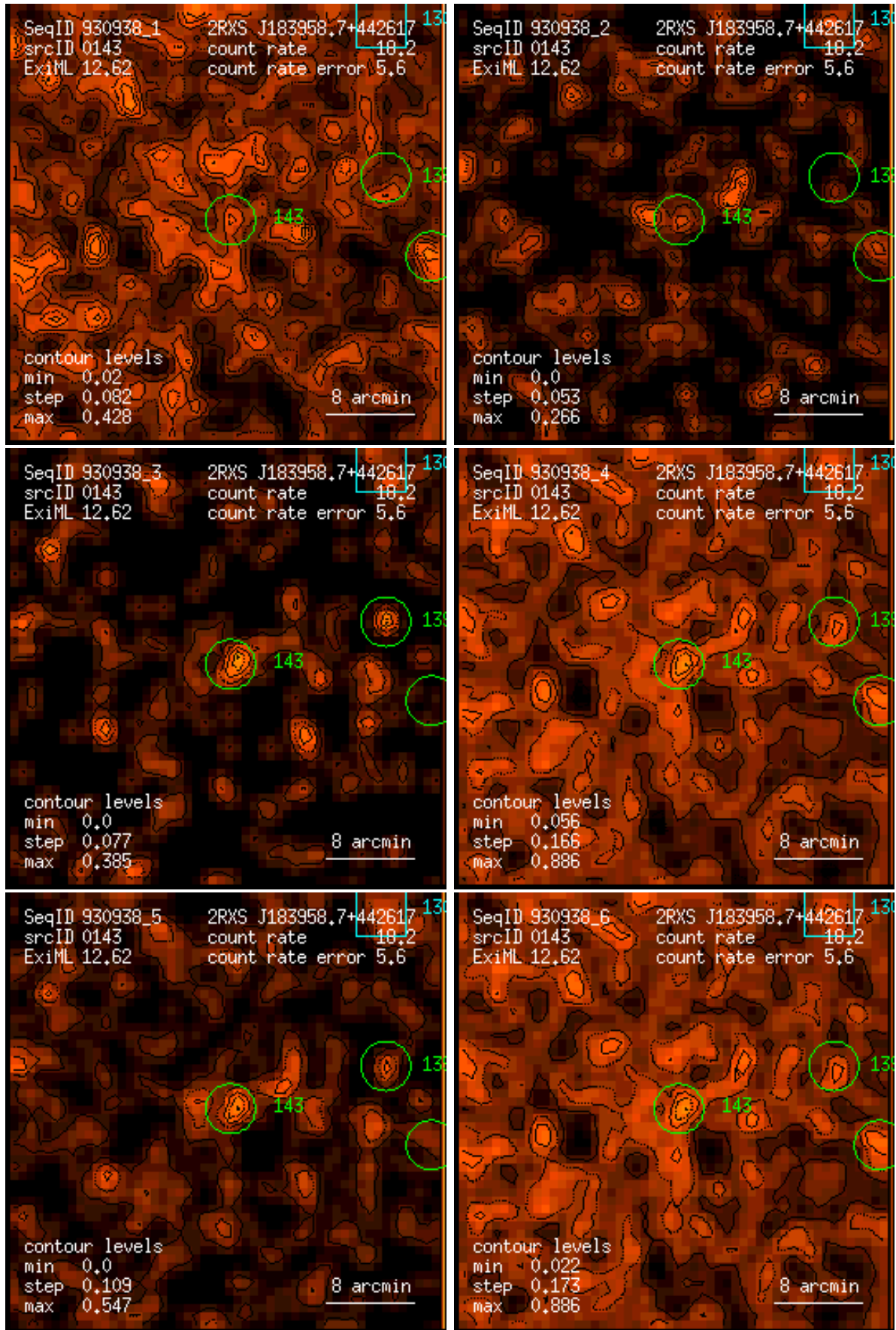
Figure 143: RASS 930938: detection 0143: band rate images, Gaussian filter: (1) PSPC channels 11 – 41, (2) 52 – 90, (3) 91 – 201, (4) 11 – 235, (5) 52 – 201, (6) 11 – 201. Broad band rates in counts/ks. Band rate contour levels in counts/ks/arcmin 2 .
