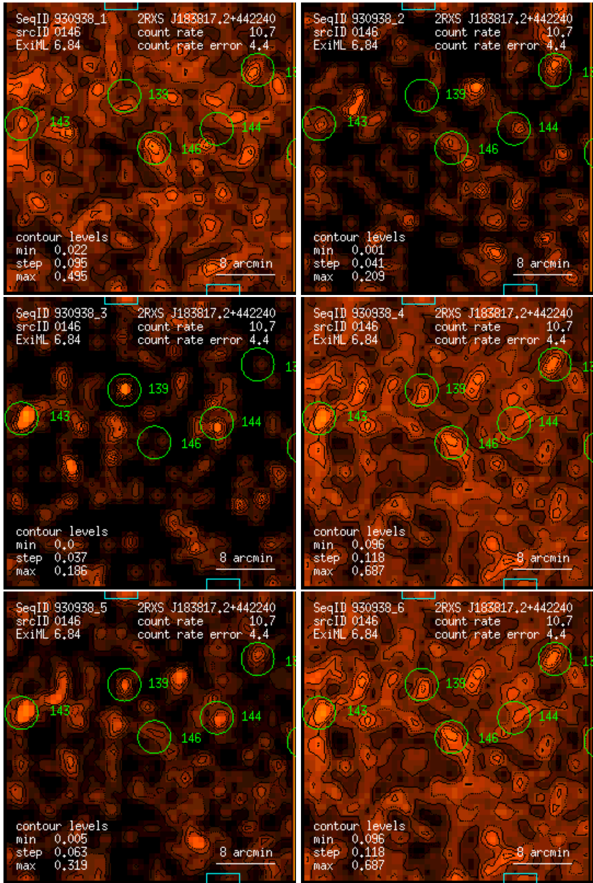
Figure 146: RASS 930938: detection 0146: band rate images, Gaussian filter: (1) PSPC channels 11 – 41, (2) 52 – 90, (3) 91 – 201, (4) 11 – 235, (5) 52 – 201, (6) 11 – 201. Broad band rates in counts/ks. Band rate contour levels in counts/ks/arcmin 2 .
