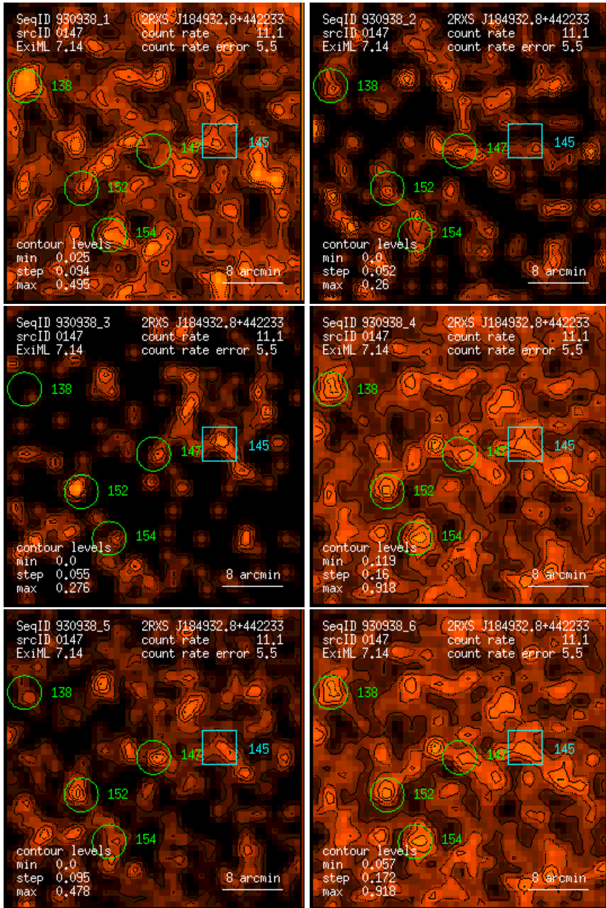
Figure 147: RASS 930938: detection 0147: band rate images, Gaussian filter: (1) PSPC channels 11 – 41, (2) 52 – 90, (3) 91 – 201, (4) 11 – 235, (5) 52 – 201, (6) 11 – 201. Broad band rates in counts/ks. Band rate contour levels in counts/ks/arcmin 2 .
