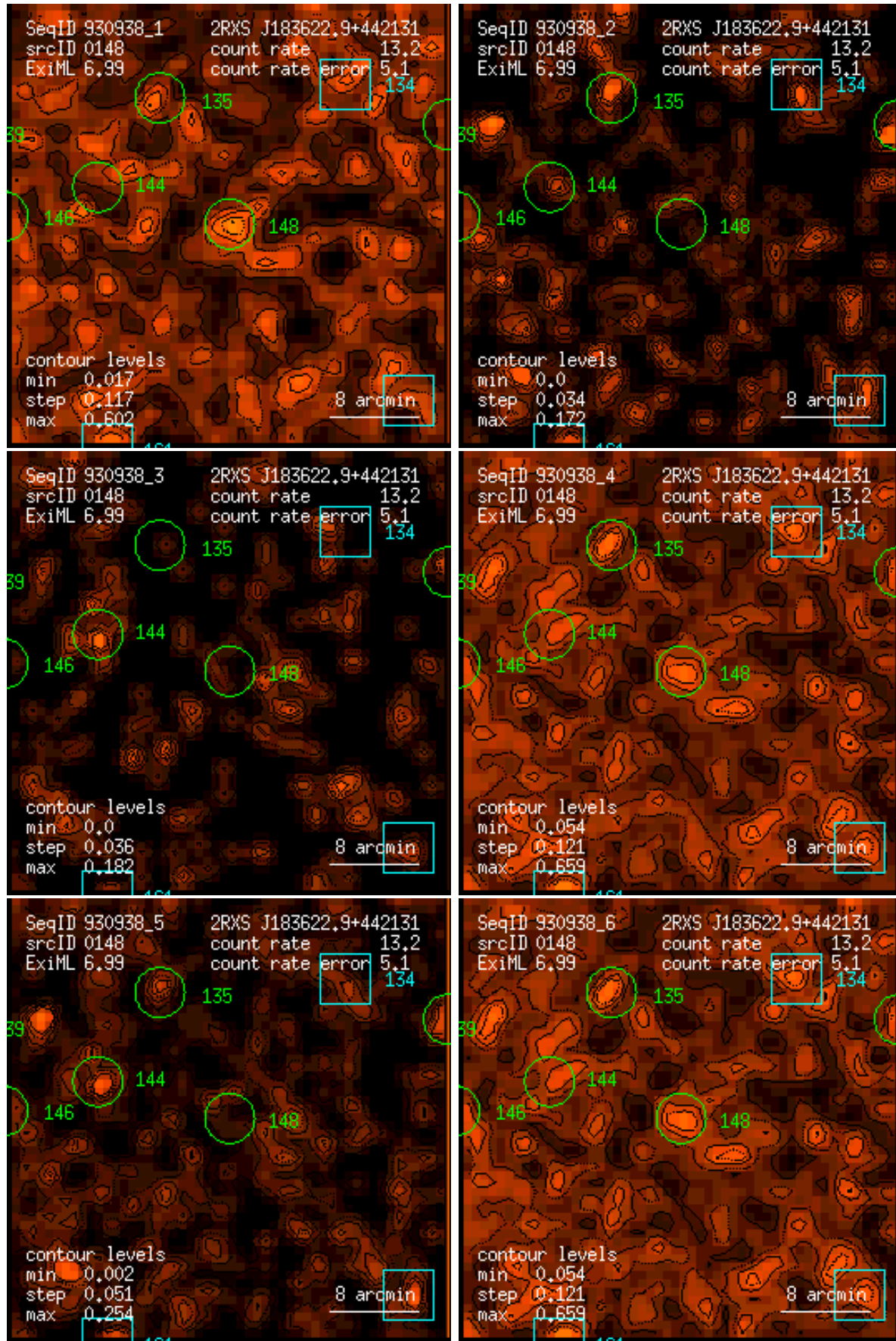
Figure 148: RASS 930938: detection 0148: band rate images, Gaussian filter: (1) PSPC channels 11 – 41, (2) 52 – 90, (3) 91 – 201, (4) 11 – 235, (5) 52 – 201, (6) 11 – 201. Broad band rates in counts/ks. Band rate contour levels in counts/ks/arcmin 2 .
