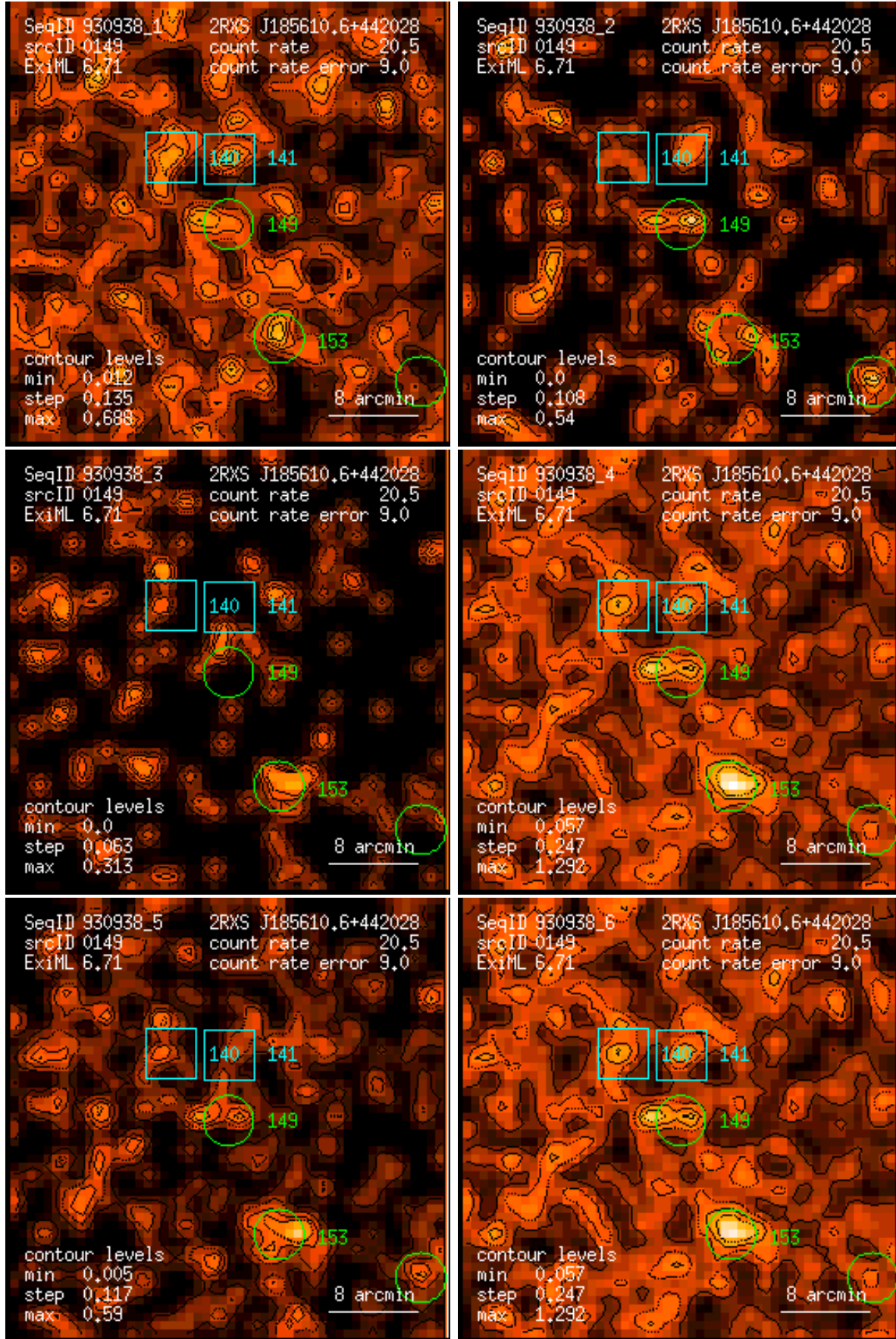
Figure 149: RASS 930938: detection 0149: band rate images, Gaussian filter: (1) PSPC channels 11 – 41, (2) 52 – 90, (3) 91 – 201, (4) 11 – 235, (5) 52 – 201, (6) 11 – 201. Broad band rates in counts/ks. Band rate contour levels in counts/ks/arcmin 2 .
