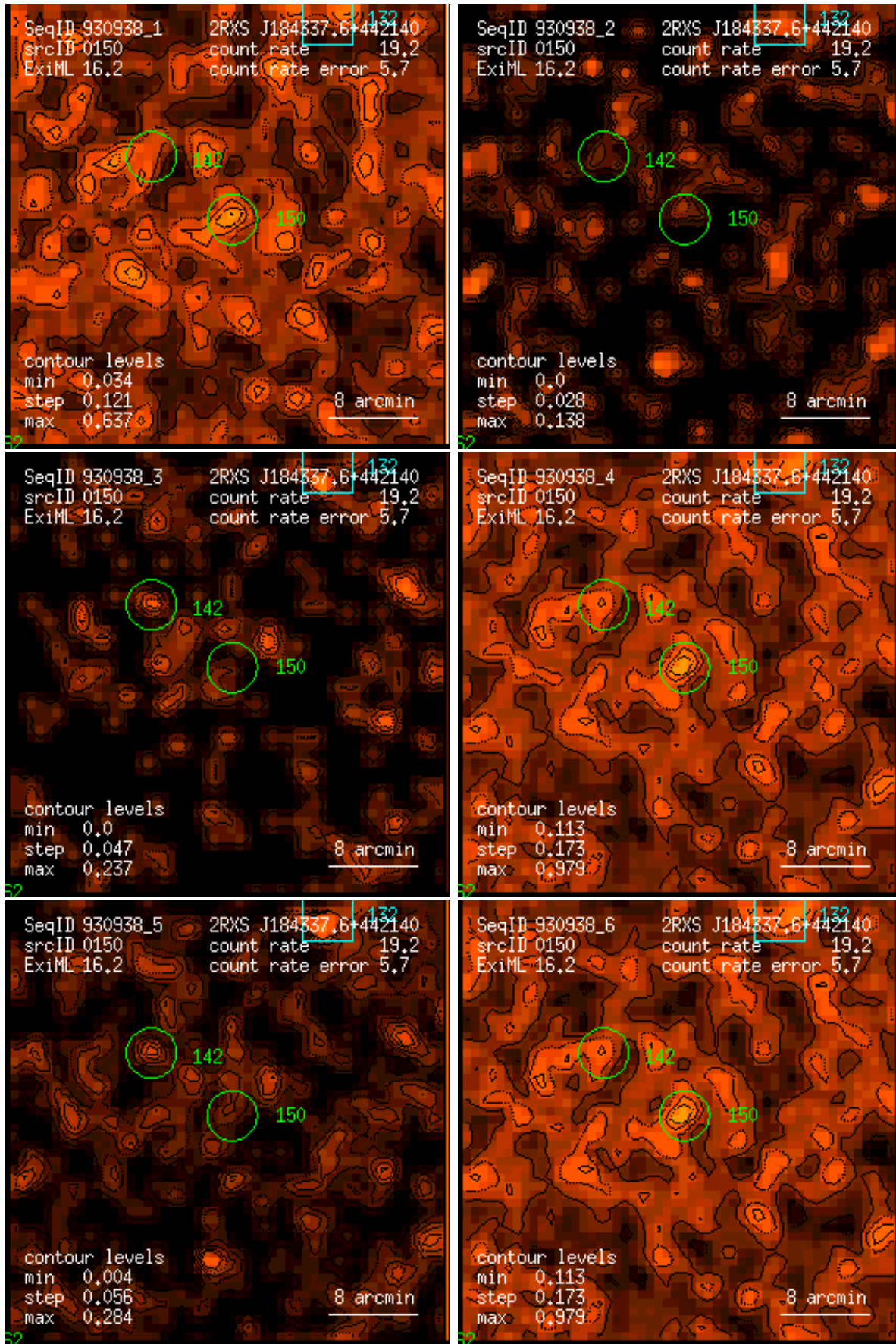
Figure 150: RASS 930938: detection 0150: band rate images, Gaussian filter: (1) PSPC channels 11 – 41, (2) 52 – 90, (3) 91 – 201, (4) 11 – 235, (5) 52 – 201, (6) 11 – 201. Broad band rates in counts/ks. Band rate contour levels in counts/ks/arcmin 2 .
