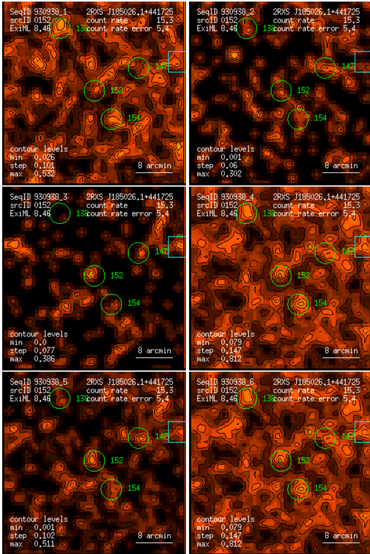
Figure 152: RASS 930938: detection 0152: band rate images, Gaussian filter: (1) PSPC channels 11 – 41, (2) 52 – 90, (3) 91 – 201, (4) 11 – 235, (5) 52 – 201, (6) 11 – 201. Broad band rates in counts/ks. Band rate contour levels in counts/ks/arcmin 2 .
