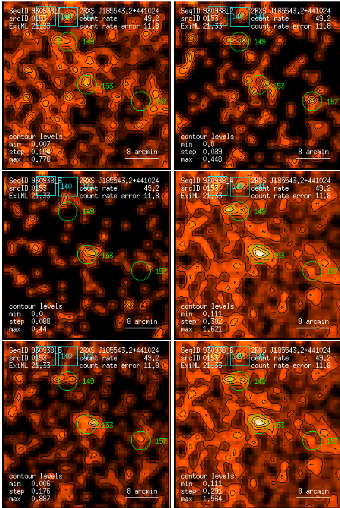
Figure 153: RASS 930938: detection 0153: band rate images, Gaussian filter: (1) PSPC channels 11 – 41, (2) 52 – 90, (3) 91 – 201, (4) 11 – 235, (5) 52 – 201, (6) 11 – 201. Broad band rates in counts/ks. Band rate contour levels in counts/ks/arcmin 2 .
