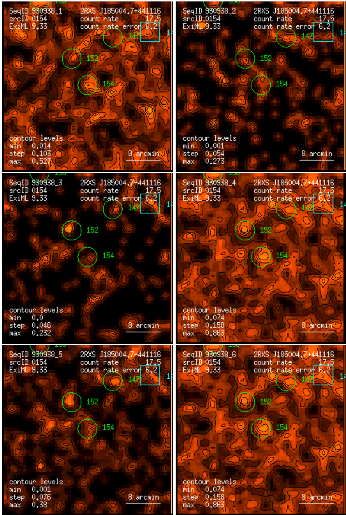
Figure 154: RASS 930938: detection 0154: band rate images, Gaussian filter: (1) PSPC channels 11 – 41, (2) 52 – 90, (3) 91 – 201, (4) 11 – 235, (5) 52 – 201, (6) 11 – 201. Broad band rates in counts/ks. Band rate contour levels in counts/ks/arcmin 2 .
