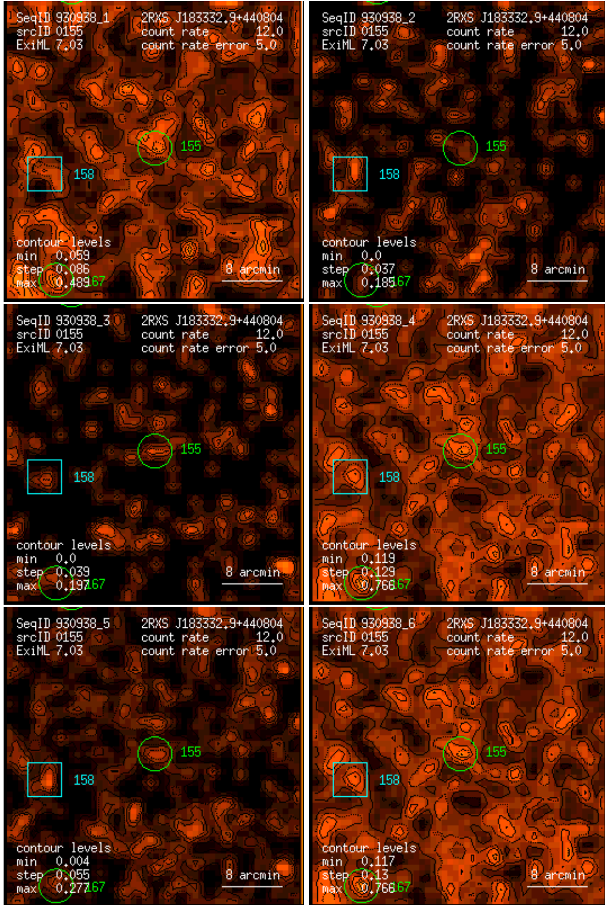
Figure 155: RASS 930938: detection 0155: band rate images, Gaussian filter: (1) PSPC channels 11 – 41, (2) 52 – 90, (3) 91 – 201, (4) 11 – 235, (5) 52 – 201, (6) 11 – 201. Broad band rates in counts/ks. Band rate contour levels in counts/ks/arcmin 2 .
