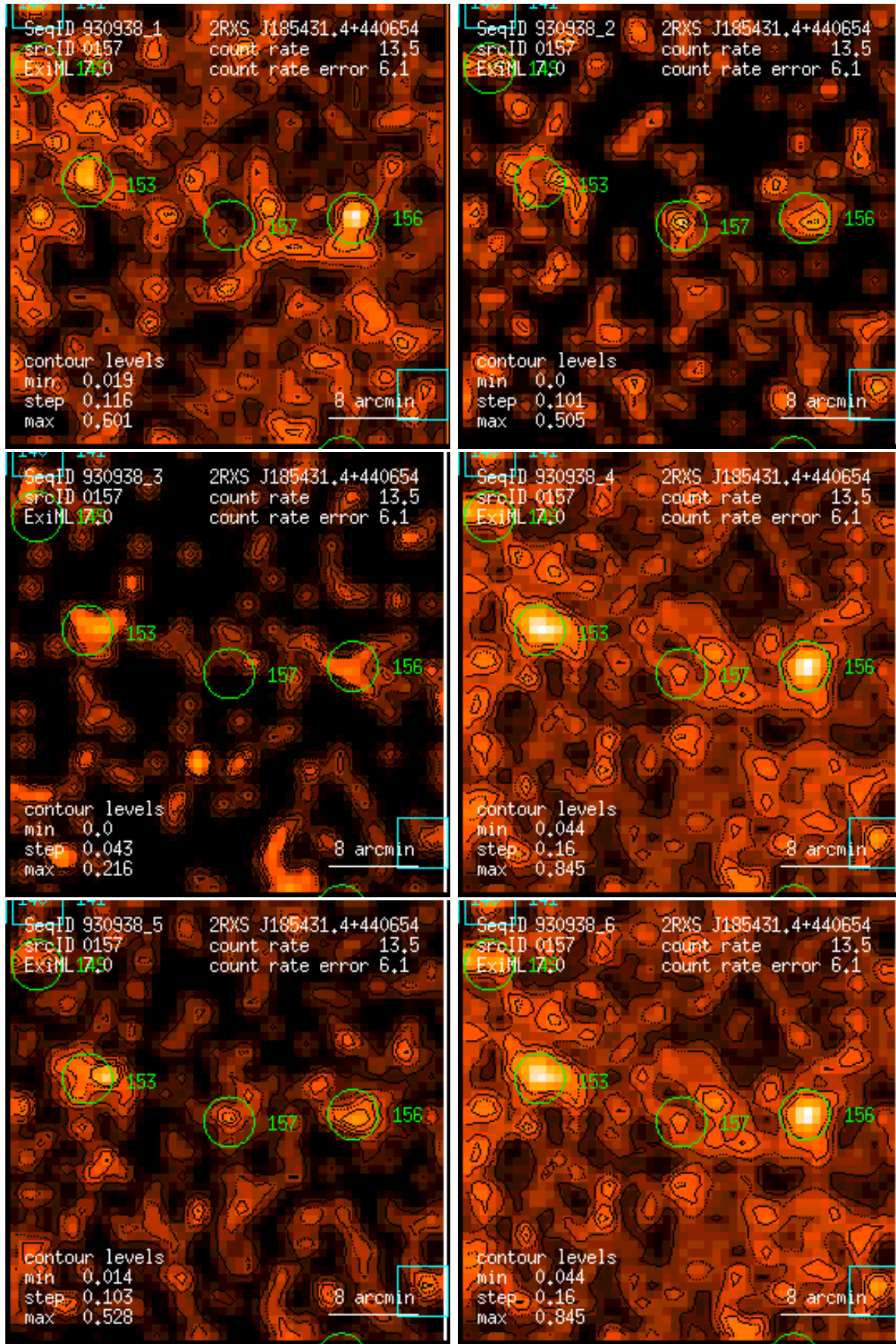
Figure 157: RASS 930938: detection 0157: band rate images, Gaussian filter: (1) PSPC channels 11 – 41, (2) 52 – 90, (3) 91 – 201, (4) 11 – 235, (5) 52 – 201, (6) 11 – 201. Broad band rates in counts/ks. Band rate contour levels in counts/ks/arcmin 2 .
