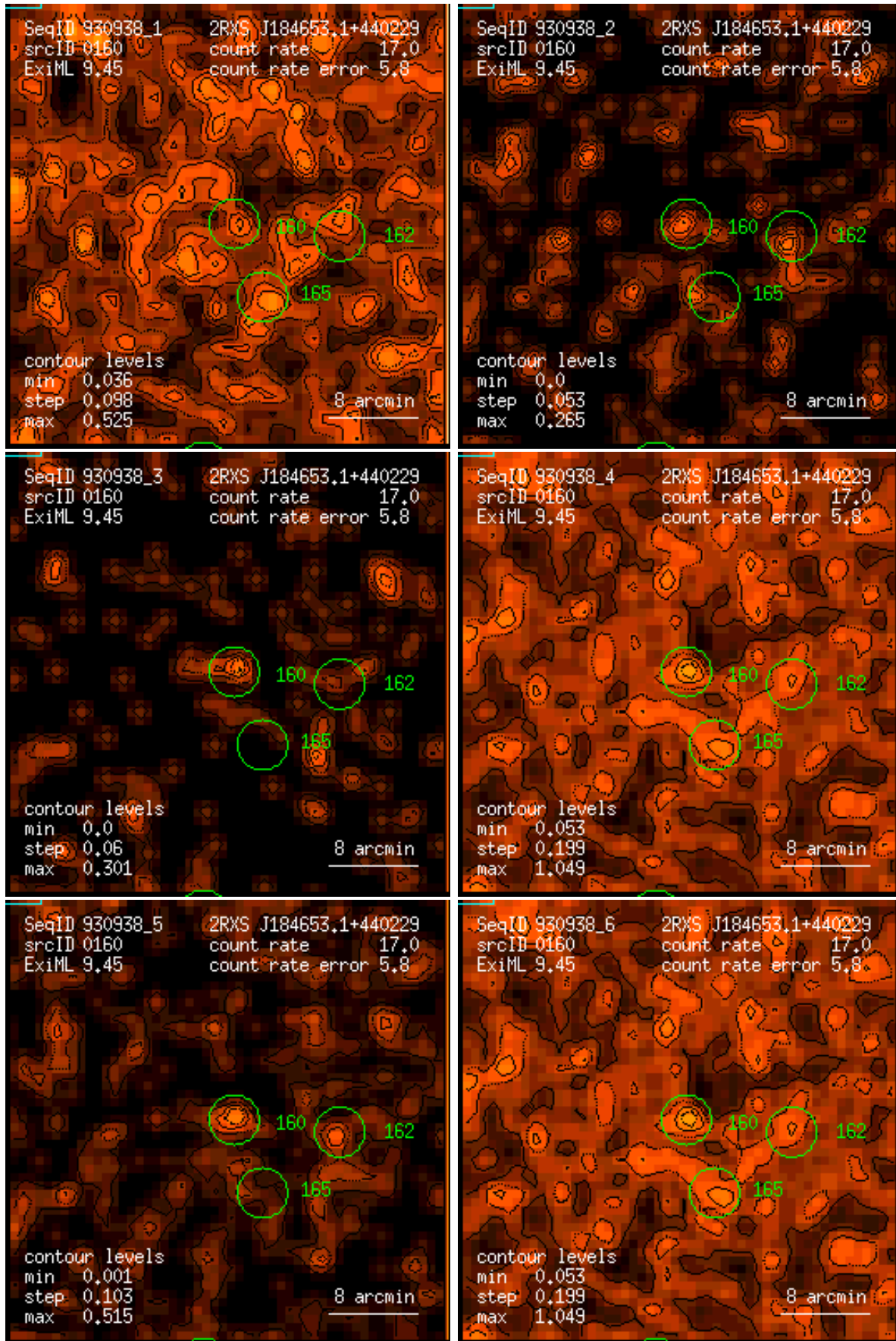
Figure 160: RASS 930938: detection 0160: band rate images, Gaussian filter: (1) PSPC channels 11 – 41, (2) 52 – 90, (3) 91 – 201, (4) 11 – 235, (5) 52 – 201, (6) 11 – 201. Broad band rates in counts/ks. Band rate contour levels in counts/ks/arcmin 2 .
