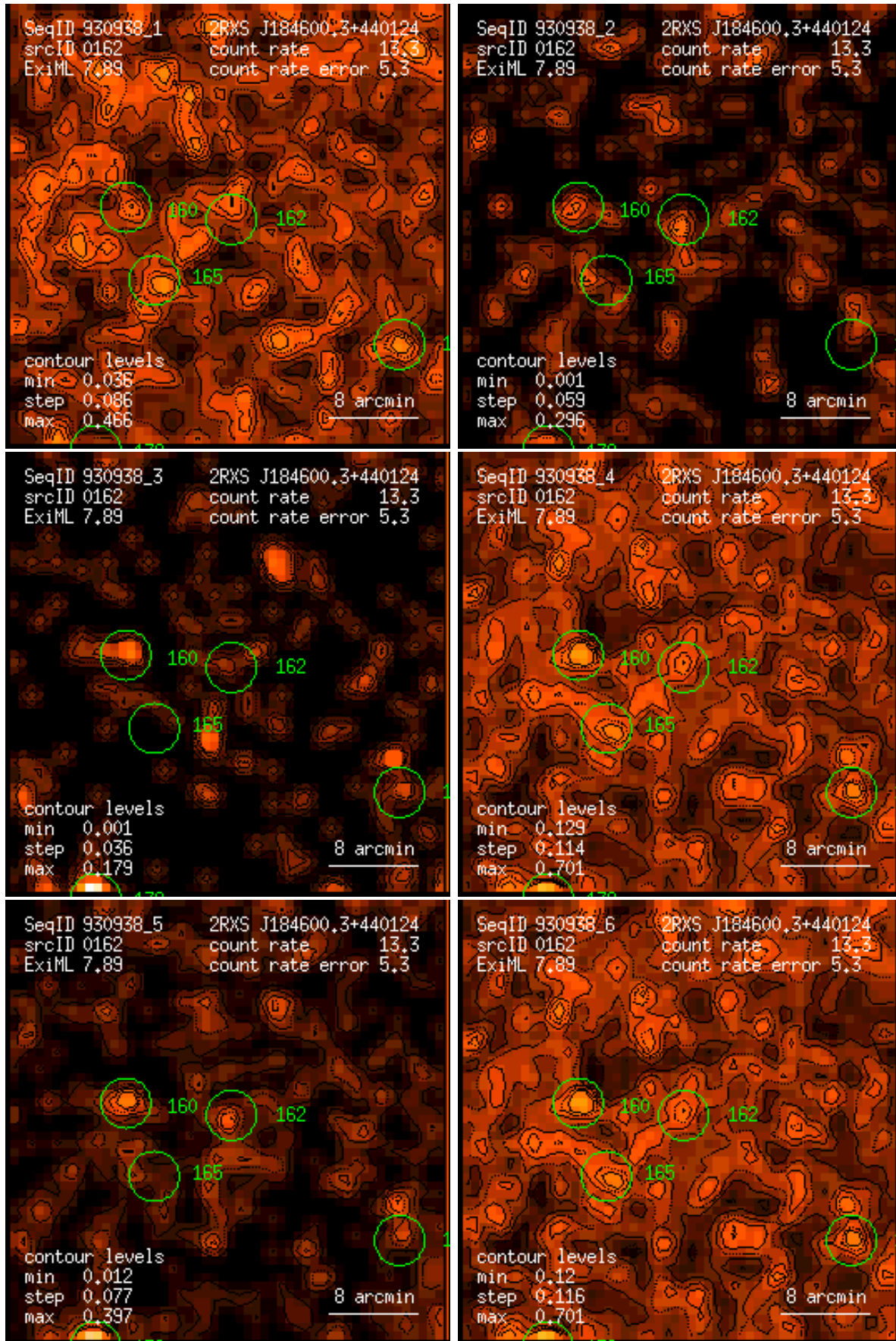
Figure 162: RASS 930938: detection 0162: band rate images, Gaussian filter: (1) PSPC channels 11 – 41, (2) 52 – 90, (3) 91 – 201, (4) 11 – 235, (5) 52 – 201, (6) 11 – 201. Broad band rates in counts/ks. Band rate contour levels in counts/ks/arcmin 2 .
