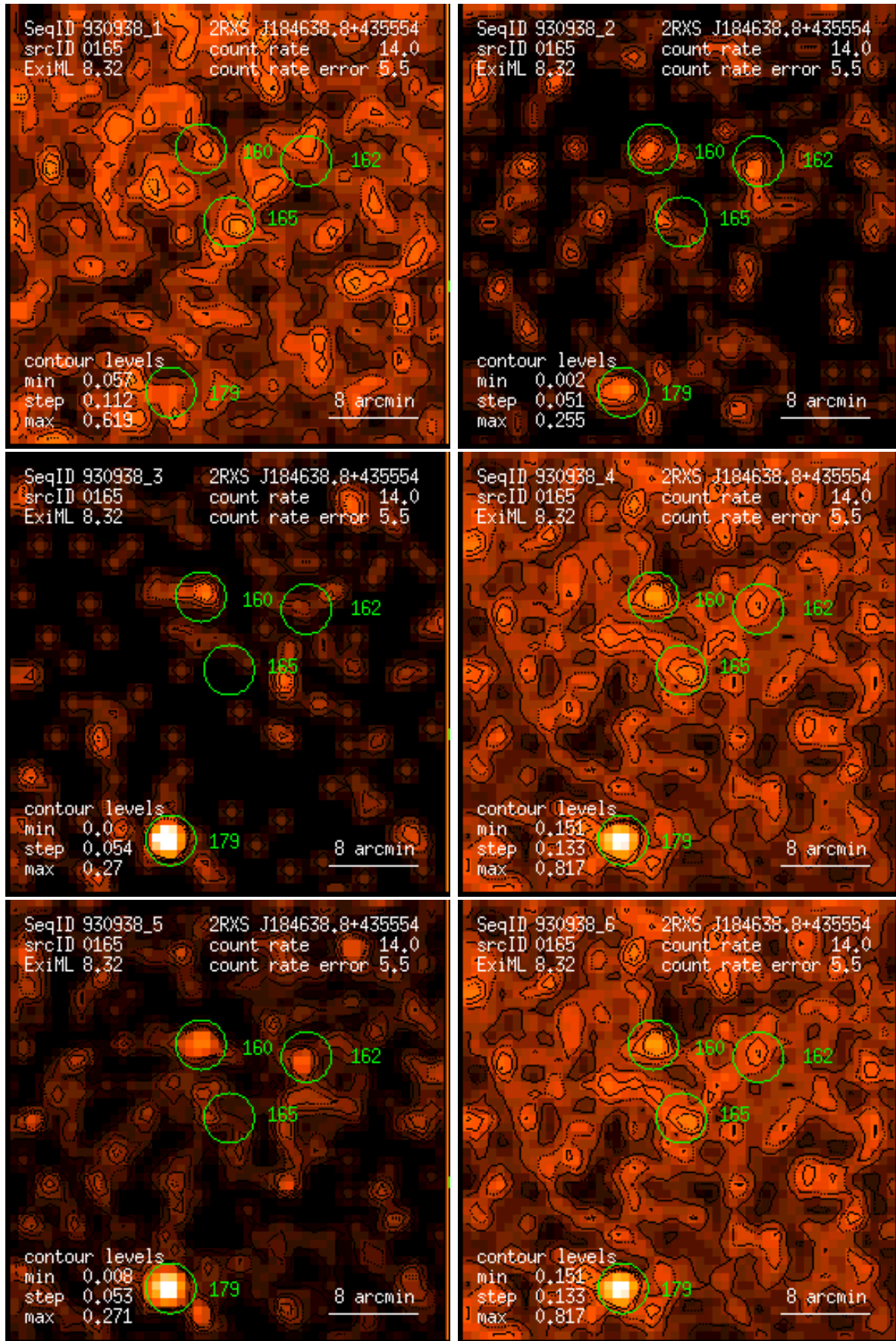
Figure 165: RASS 930938: detection 0165: band rate images, Gaussian filter: (1) PSPC channels 11 – 41, (2) 52 – 90, (3) 91 – 201, (4) 11 – 235, (5) 52 – 201, (6) 11 – 201. Broad band rates in counts/ks. Band rate contour levels in counts/ks/arcmin 2 .
