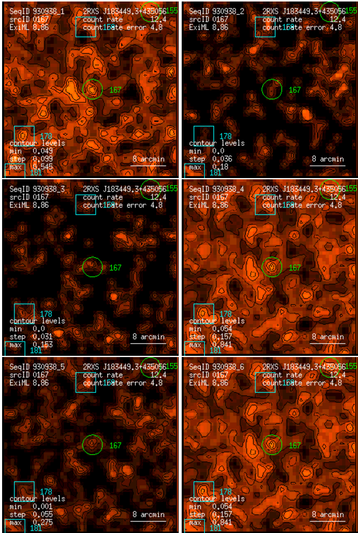
Figure 167: RASS 930938: detection 0167: band rate images, Gaussian filter: (1) PSPC channels 11 – 41, (2) 52 – 90, (3) 91 – 201, (4) 11 – 235, (5) 52 – 201, (6) 11 – 201. Broad band rates in counts/ks. Band rate contour levels in counts/ks/arcmin 2 .
