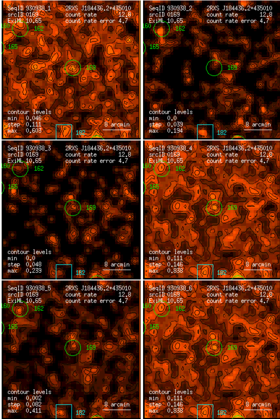
Figure 169: RASS 930938: detection 0169: band rate images, Gaussian filter: (1) PSPC channels 11 – 41, (2) 52 – 90, (3) 91 – 201, (4) 11 – 235, (5) 52 – 201, (6) 11 – 201. Broad band rates in counts/ks. Band rate contour levels in counts/ks/arcmin 2 .
