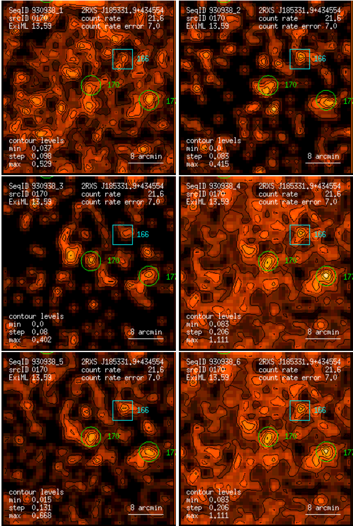
Figure 170: RASS 930938: detection 0170: band rate images, Gaussian filter: (1) PSPC channels 11 – 41, (2) 52 – 90, (3) 91 – 201, (4) 11 – 235, (5) 52 – 201, (6) 11 – 201. Broad band rates in counts/ks. Band rate contour levels in counts/ks/arcmin 2 .
