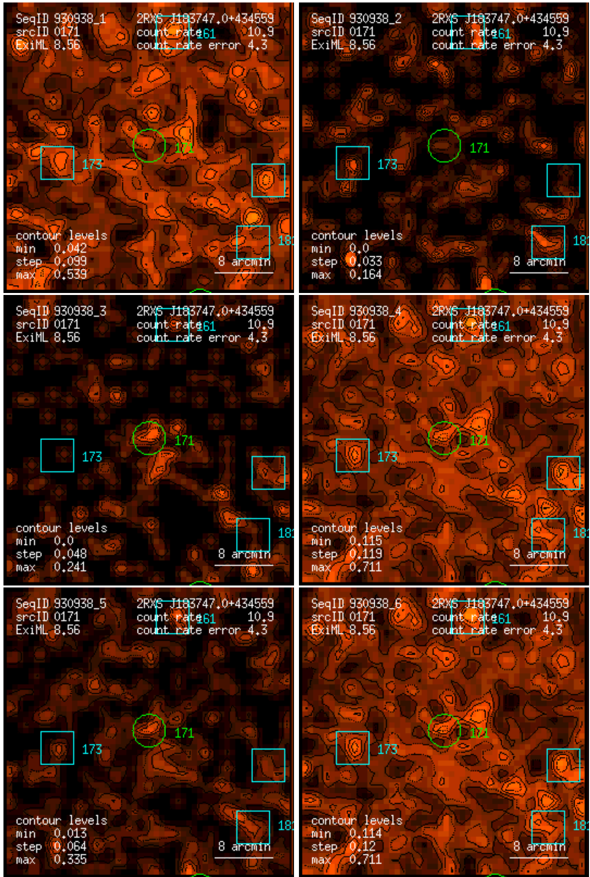
Figure 171: RASS 930938: detection 0171: band rate images, Gaussian filter: (1) PSPC channels 11 – 41, (2) 52 – 90, (3) 91 – 201, (4) 11 – 235, (5) 52 – 201, (6) 11 – 201. Broad band rates in counts/ks. Band rate contour levels in counts/ks/arcmin 2 .
