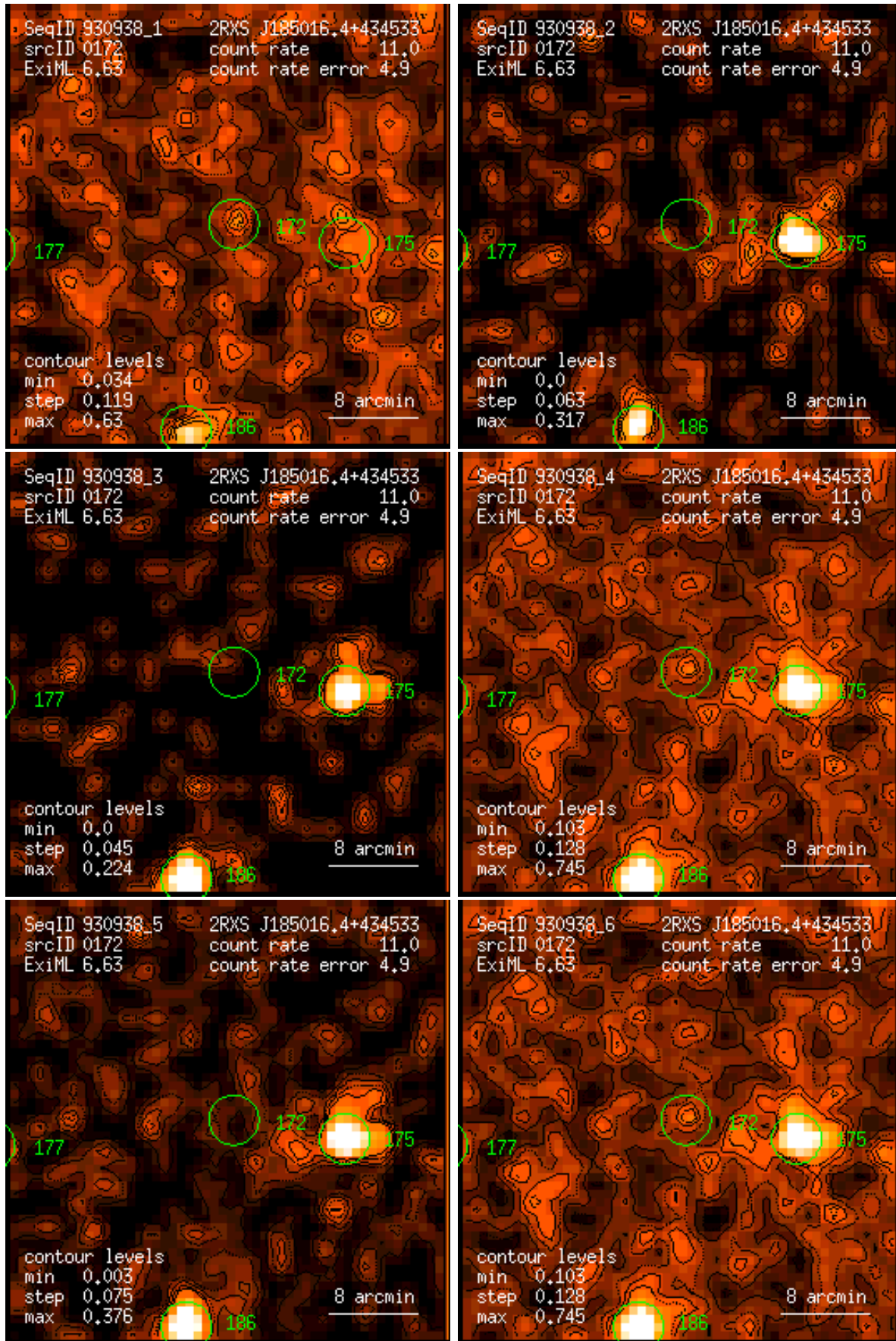
Figure 172: RASS 930938: detection 0172: band rate images, Gaussian filter: (1) PSPC channels 11 – 41, (2) 52 – 90, (3) 91 – 201, (4) 11 – 235, (5) 52 – 201, (6) 11 – 201. Broad band rates in counts/ks. Band rate contour levels in counts/ks/arcmin 2 .
