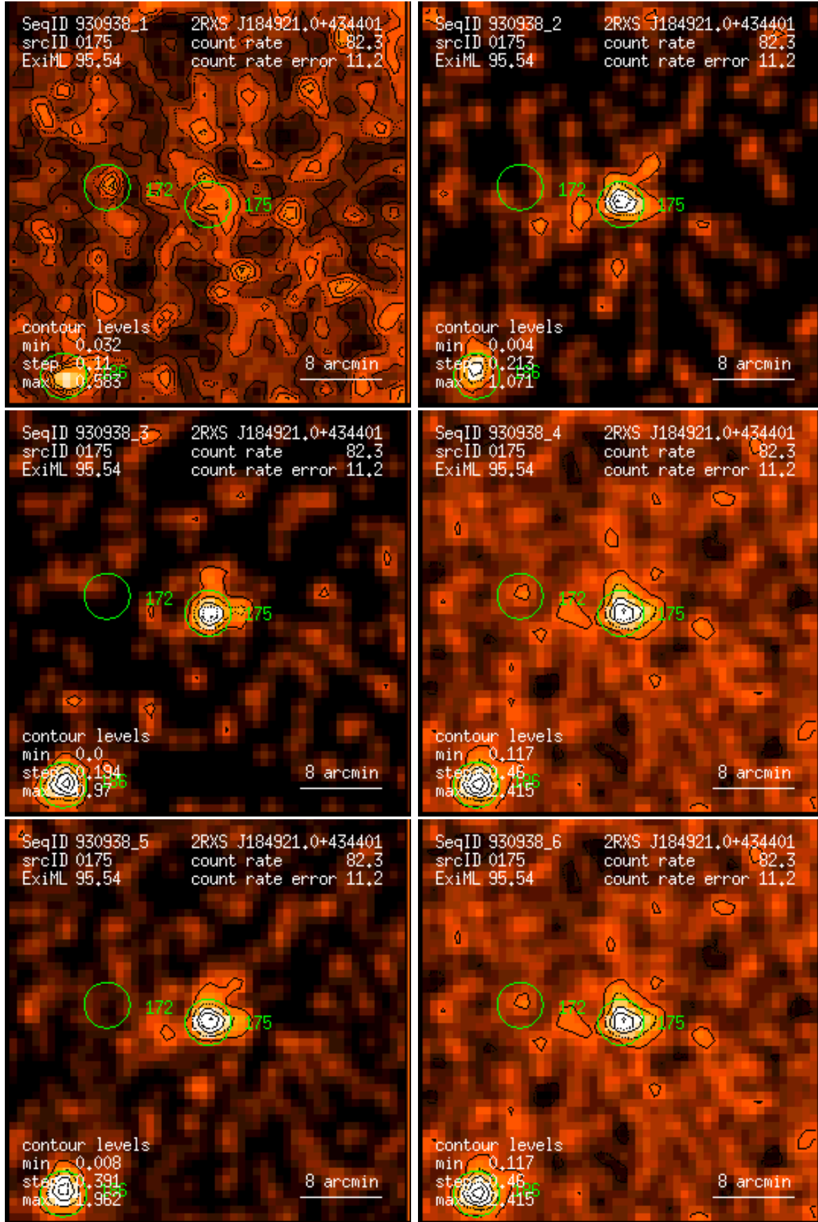
Figure 175: RASS 930938: detection 0175: band rate images, Gaussian filter: (1) PSPC channels 11 – 41, (2) 52 – 90, (3) 91 – 201, (4) 11 – 235, (5) 52 – 201, (6) 11 – 201. Broad band rates in counts/ks. Band rate contour levels in counts/ks/arcmin 2 .
