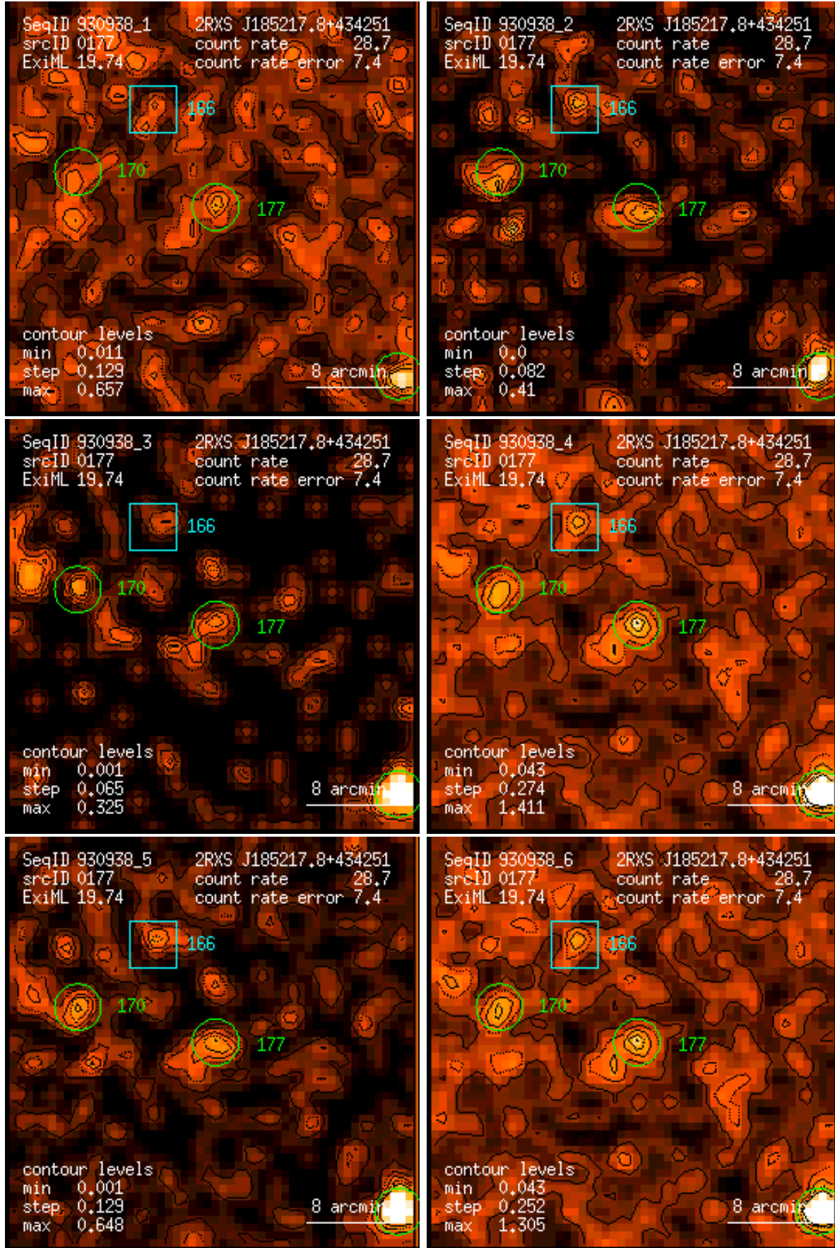
Figure 177: RASS 930938: detection 0177: band rate images, Gaussian filter: (1) PSPC channels 11 – 41, (2) 52 – 90, (3) 91 – 201, (4) 11 – 235, (5) 52 – 201, (6) 11 – 201. Broad band rates in counts/ks. Band rate contour levels in counts/ks/arcmin 2 .
