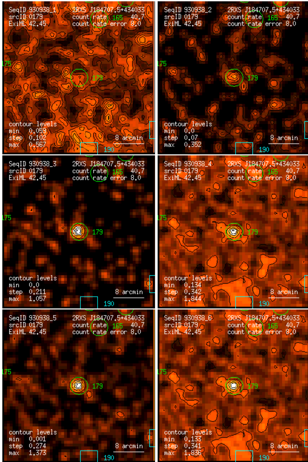
Figure 179: RASS 930938: detection 0179: band rate images, Gaussian filter: (1) PSPC channels 11 – 41, (2) 52 – 90, (3) 91 – 201, (4) 11 – 235, (5) 52 – 201, (6) 11 – 201. Broad band rates in counts/ks. Band rate contour levels in counts/ks/arcmin 2 .
