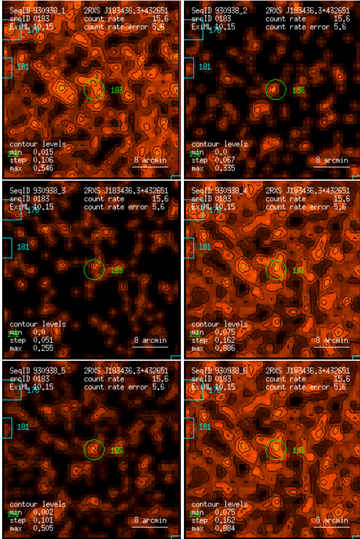
Figure 183: RASS 930938: detection 0183: band rate images, Gaussian filter: (1) PSPC channels 11 – 41, (2) 52 – 90, (3) 91 – 201, (4) 11 – 235, (5) 52 – 201, (6) 11 – 201. Broad band rates in counts/ks. Band rate contour levels in counts/ks/arcmin 2 .
