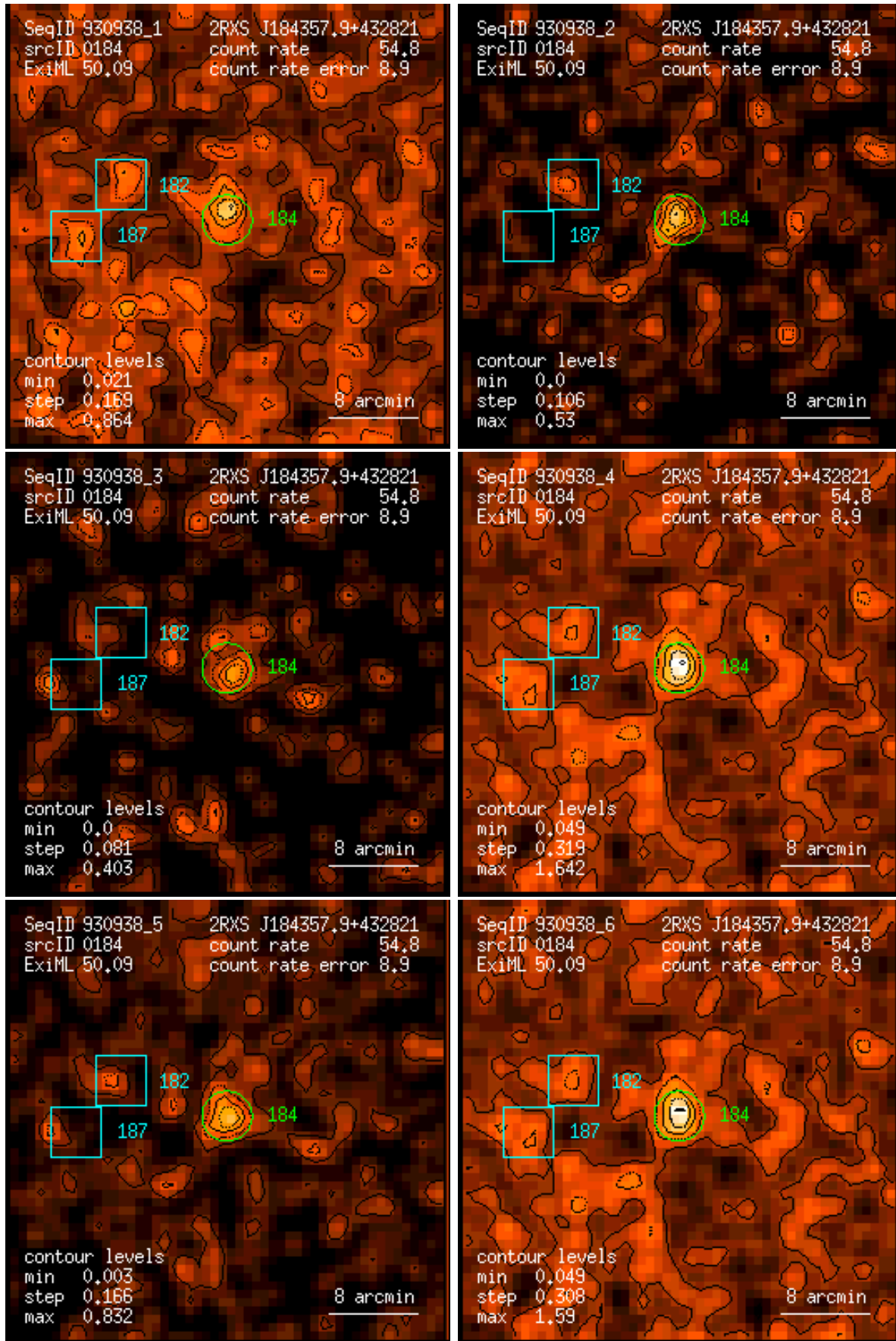
Figure 184: RASS 930938: detection 0184: band rate images, Gaussian filter: (1) PSPC channels 11 – 41, (2) 52 – 90, (3) 91 – 201, (4) 11 – 235, (5) 52 – 201, (6) 11 – 201. Broad band rates in counts/ks. Band rate contour levels in counts/ks/arcmin 2 .
