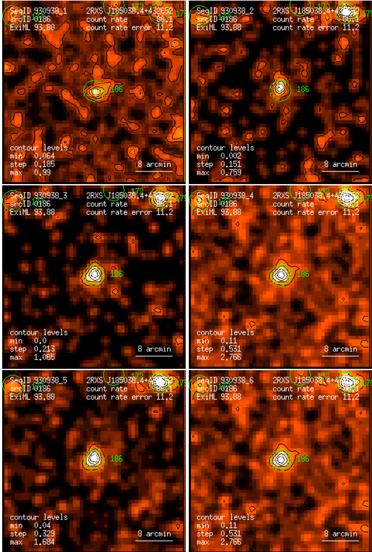
Figure 186: RASS 930938: detection 0186: band rate images, Gaussian filter: (1) PSPC channels 11 – 41, (2) 52 – 90, (3) 91 – 201, (4) 11 – 235, (5) 52 – 201, (6) 11 – 201. Broad band rates in counts/ks. Band rate contour levels in counts/ks/arcmin 2 .
