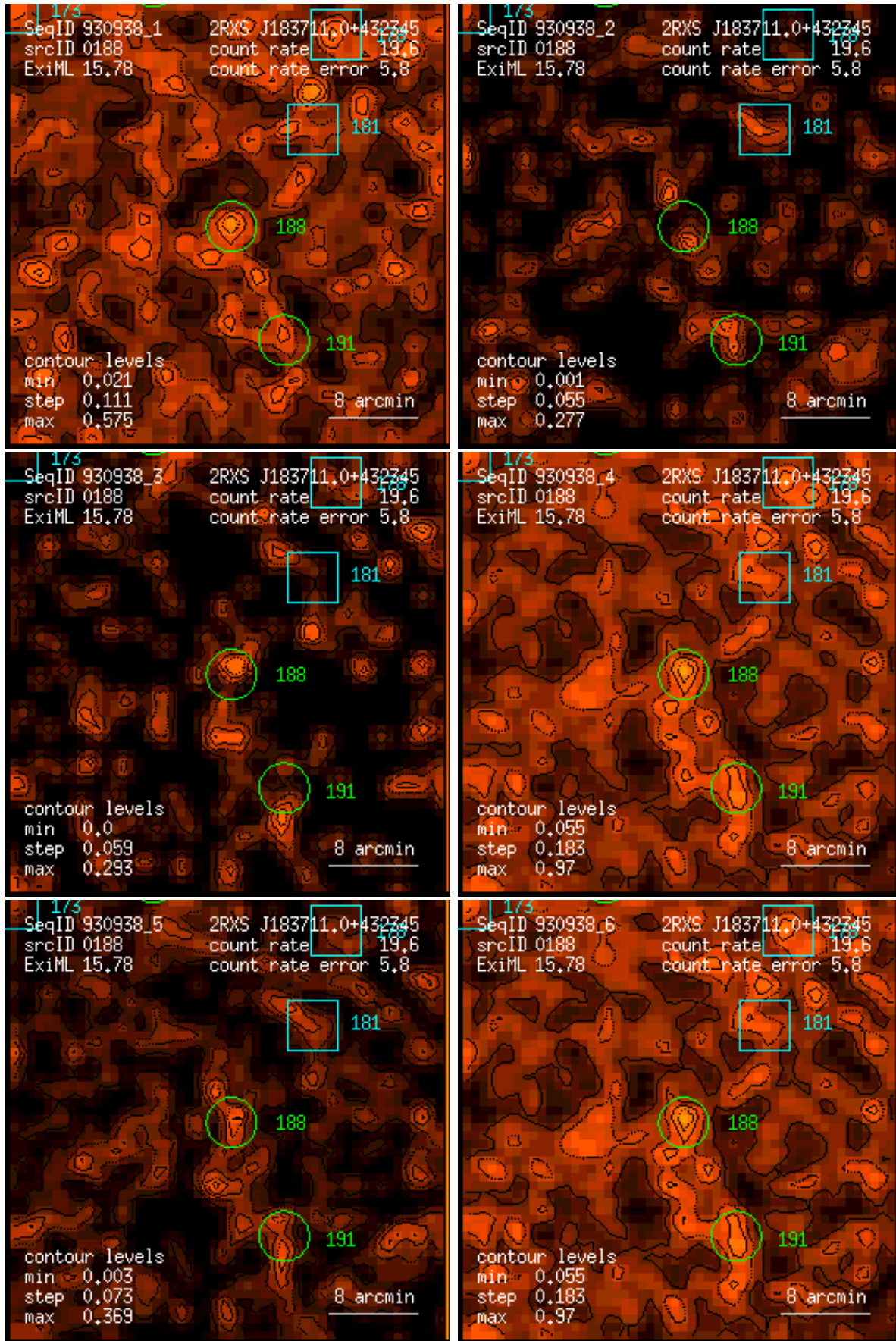
Figure 188: RASS 930938: detection 0188: band rate images, Gaussian filter: (1) PSPC channels 11 – 41, (2) 52 – 90, (3) 91 – 201, (4) 11 – 235, (5) 52 – 201, (6) 11 – 201. Broad band rates in counts/ks. Band rate contour levels in counts/ks/arcmin 2 .
