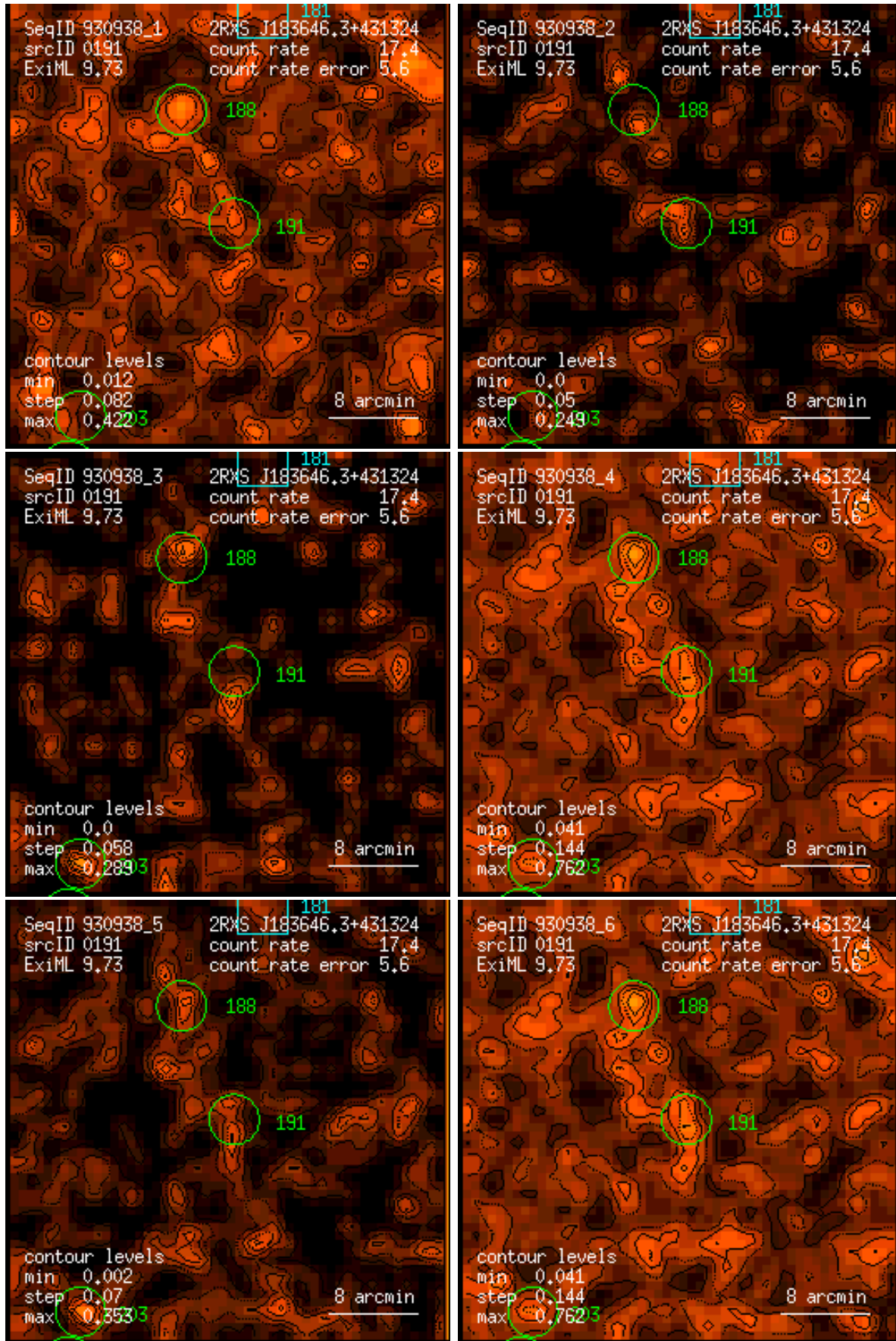
Figure 191: RASS 930938: detection 0191: band rate images, Gaussian filter: (1) PSPC channels 11 – 41, (2) 52 – 90, (3) 91 – 201, (4) 11 – 235, (5) 52 – 201, (6) 11 – 201. Broad band rates in counts/ks. Band rate contour levels in counts/ks/arcmin 2 .
