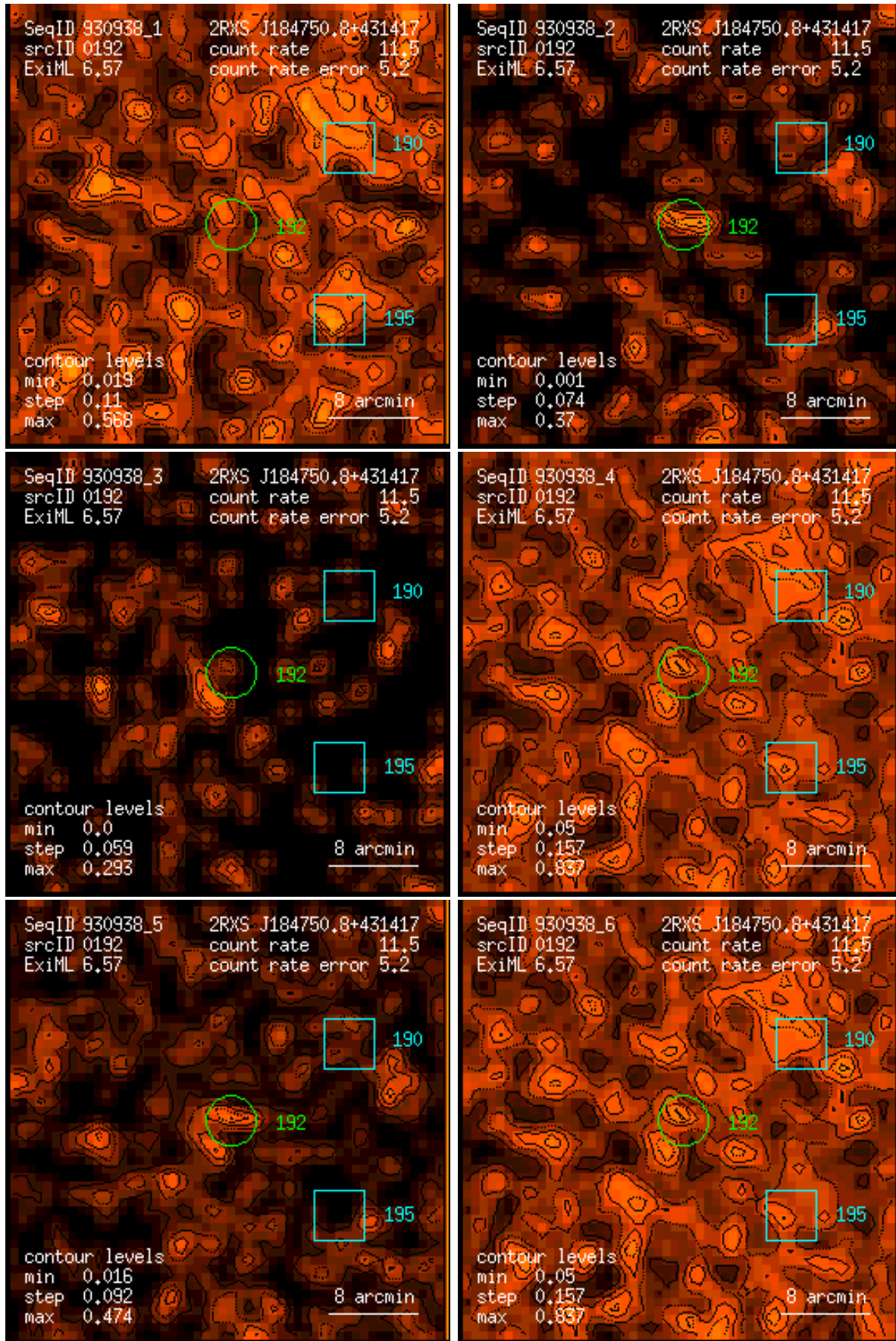
Figure 192: RASS 930938: detection 0192: band rate images, Gaussian filter: (1) PSPC channels 11 – 41, (2) 52 – 90, (3) 91 – 201, (4) 11 – 235, (5) 52 – 201, (6) 11 – 201. Broad band rates in counts/ks. Band rate contour levels in counts/ks/arcmin 2 .
