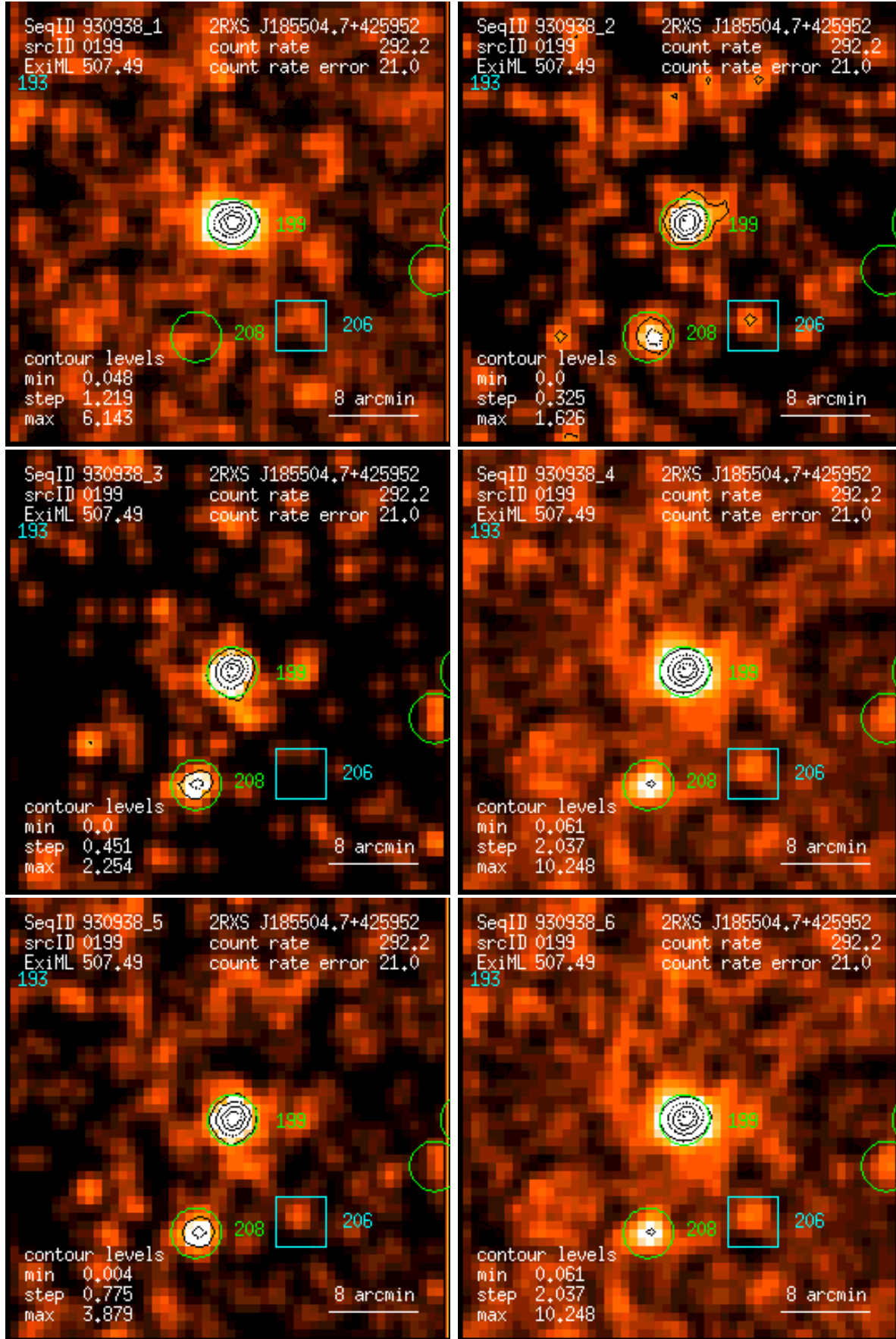
Figure 199: RASS 930938: detection 0199: band rate images, Gaussian filter: (1) PSPC channels 11 – 41, (2) 52 – 90, (3) 91 – 201, (4) 11 – 235, (5) 52 – 201, (6) 11 – 201. Broad band rates in counts/ks. Band rate contour levels in counts/ks/arcmin 2 .
