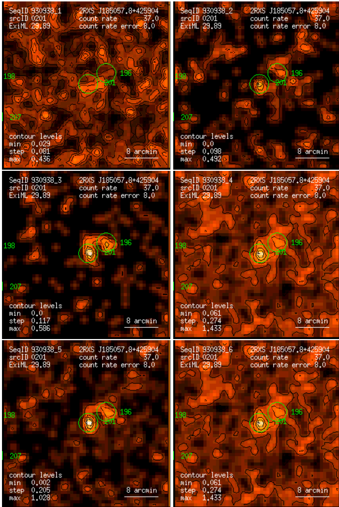
Figure 201: RASS 930938: detection 0201: band rate images, Gaussian filter: (1) PSPC channels 11 – 41, (2) 52 – 90, (3) 91 – 201, (4) 11 – 235, (5) 52 – 201, (6) 11 – 201. Broad band rates in counts/ks. Band rate contour levels in counts/ks/arcmin 2 .
