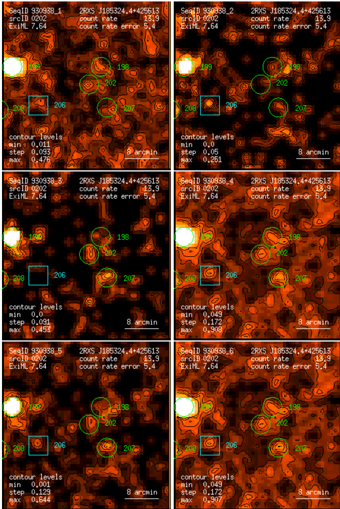
Figure 202: RASS 930938: detection 0202: band rate images, Gaussian filter: (1) PSPC channels 11 – 41, (2) 52 – 90, (3) 91 – 201, (4) 11 – 235, (5) 52 – 201, (6) 11 – 201. Broad band rates in counts/ks. Band rate contour levels in counts/ks/arcmin 2 .
