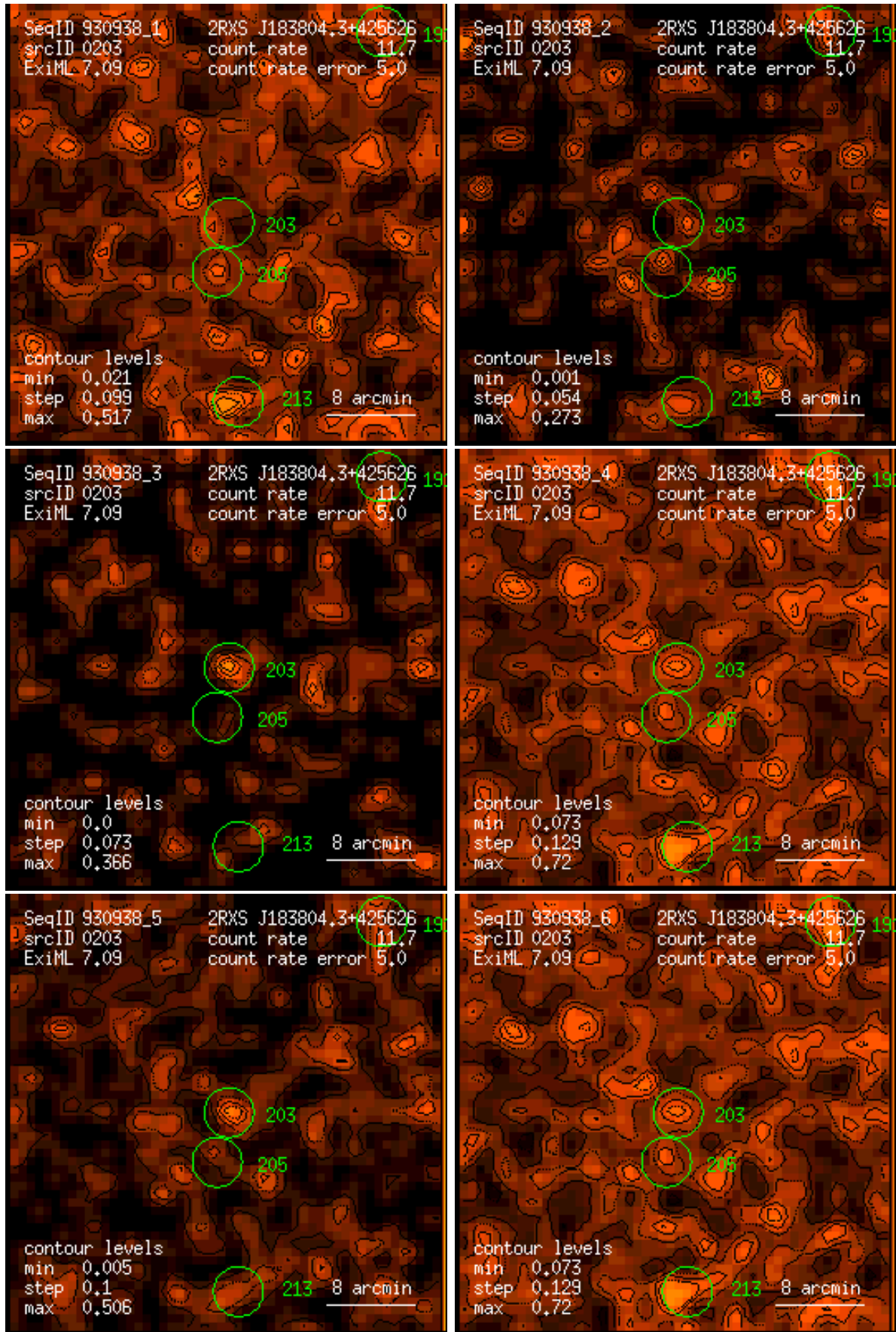
Figure 203: RASS 930938: detection 0203: band rate images, Gaussian filter: (1) PSPC channels 11 – 41, (2) 52 – 90, (3) 91 – 201, (4) 11 – 235, (5) 52 – 201, (6) 11 – 201. Broad band rates in counts/ks. Band rate contour levels in counts/ks/arcmin 2 .
