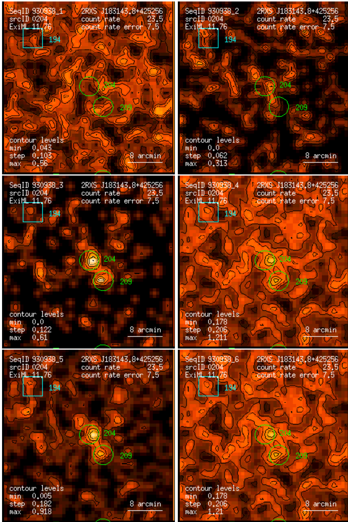
Figure 204: RASS 930938: detection 0204: band rate images, Gaussian filter: (1) PSPC channels 11 – 41, (2) 52 – 90, (3) 91 – 201, (4) 11 – 235, (5) 52 – 201, (6) 11 – 201. Broad band rates in counts/ks. Band rate contour levels in counts/ks/arcmin 2 .
