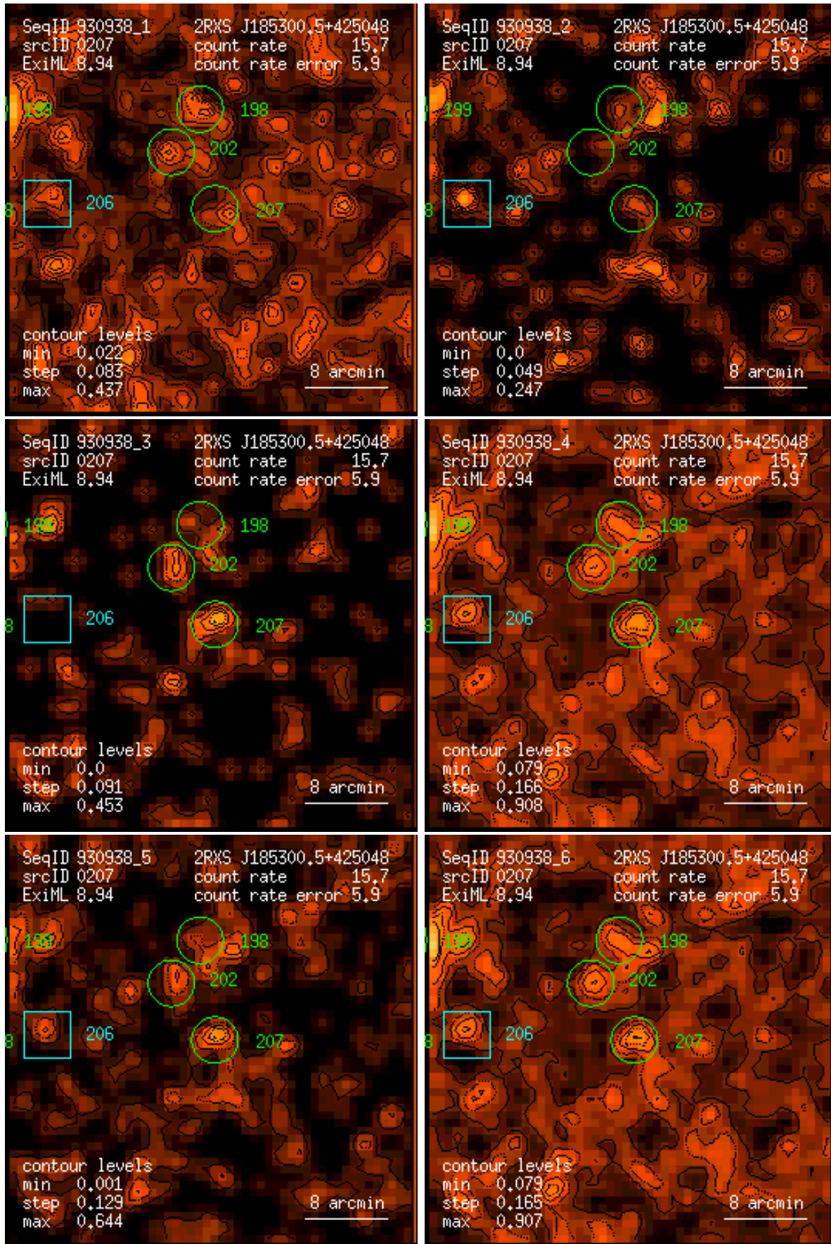
Figure 207: RASS 930938: detection 0207: band rate images, Gaussian filter: (1) PSPC channels 11 – 41, (2) 52 – 90, (3) 91 – 201, (4) 11 – 235, (5) 52 – 201, (6) 11 – 201. Broad band rates in counts/ks. Band rate contour levels in counts/ks/arcmin 2 .
