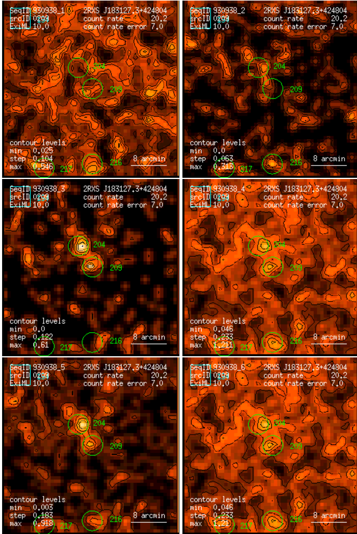
Figure 209: RASS 930938: detection 0209: band rate images, Gaussian filter: (1) PSPC channels 11 – 41, (2) 52 – 90, (3) 91 – 201, (4) 11 – 235, (5) 52 – 201, (6) 11 – 201. Broad band rates in counts/ks. Band rate contour levels in counts/ks/arcmin 2 .
