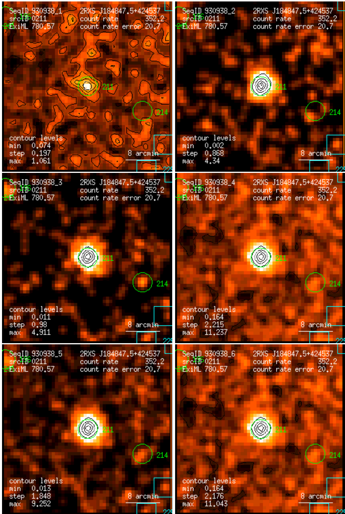
Figure 211: RASS 930938: detection 0211: band rate images, Gaussian filter: (1) PSPC channels 11 – 41, (2) 52 – 90, (3) 91 – 201, (4) 11 – 235, (5) 52 – 201, (6) 11 – 201. Broad band rates in counts/ks. Band rate contour levels in counts/ks/arcmin 2 .
