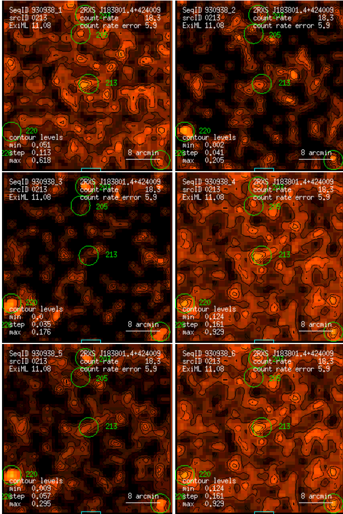
Figure 213: RASS 930938: detection 0213: band rate images, Gaussian filter: (1) PSPC channels 11 – 41, (2) 52 – 90, (3) 91 – 201, (4) 11 – 235, (5) 52 – 201, (6) 11 – 201. Broad band rates in counts/ks. Band rate contour levels in counts/ks/arcmin 2 .
