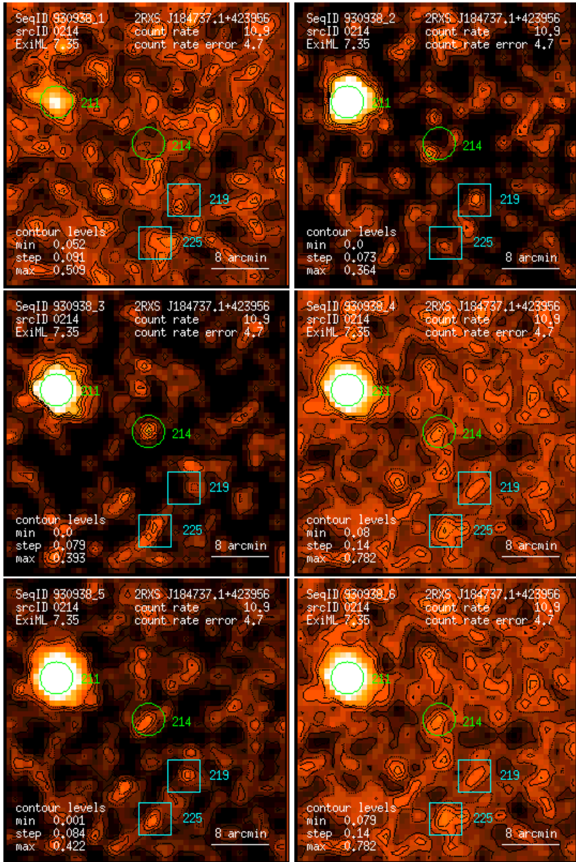
Figure 214: RASS 930938: detection 0214: band rate images, Gaussian filter: (1) PSPC channels 11 – 41, (2) 52 – 90, (3) 91 – 201, (4) 11 – 235, (5) 52 – 201, (6) 11 – 201. Broad band rates in counts/ks. Band rate contour levels in counts/ks/arcmin 2 .
