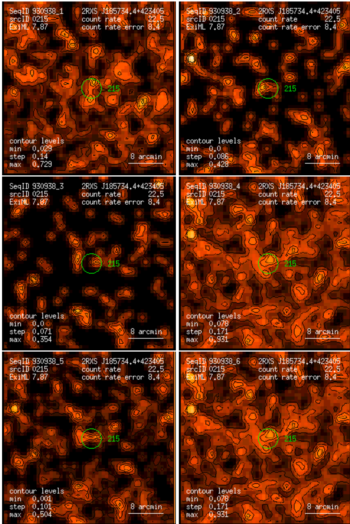
Figure 215: RASS 930938: detection 0215: band rate images, Gaussian filter: (1) PSPC channels 11 – 41, (2) 52 – 90, (3) 91 – 201, (4) 11 – 235, (5) 52 – 201, (6) 11 – 201. Broad band rates in counts/ks. Band rate contour levels in counts/ks/arcmin 2 .
