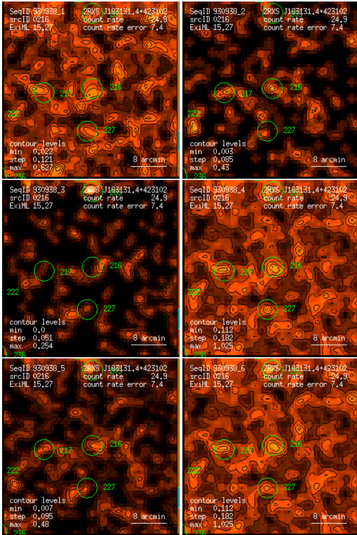
Figure 216: RASS 930938: detection 0216: band rate images, Gaussian filter: (1) PSPC channels 11 – 41, (2) 52 – 90, (3) 91 – 201, (4) 11 – 235, (5) 52 – 201, (6) 11 – 201. Broad band rates in counts/ks. Band rate contour levels in counts/ks/arcmin 2 .
