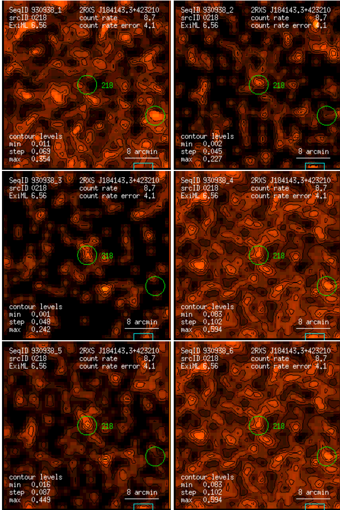
Figure 218: RASS 930938: detection 0218: band rate images, Gaussian filter: (1) PSPC channels 11 – 41, (2) 52 – 90, (3) 91 – 201, (4) 11 – 235, (5) 52 – 201, (6) 11 – 201. Broad band rates in counts/ks. Band rate contour levels in counts/ks/arcmin 2 .
