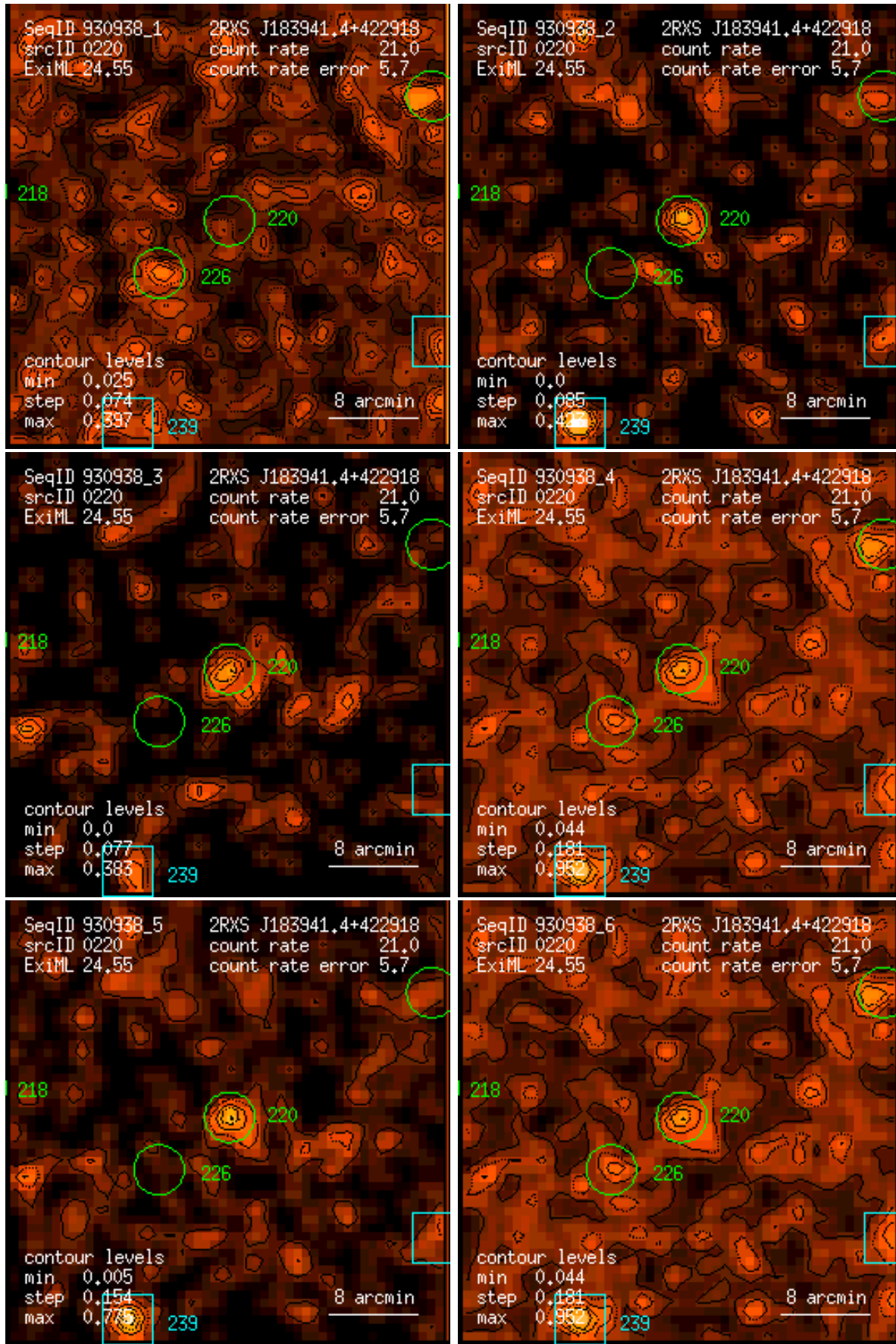
Figure 220: RASS 930938: detection 0220: band rate images, Gaussian filter: (1) PSPC channels 11 – 41, (2) 52 – 90, (3) 91 – 201, (4) 11 – 235, (5) 52 – 201, (6) 11 – 201. Broad band rates in counts/ks. Band rate contour levels in counts/ks/arcmin 2 .
