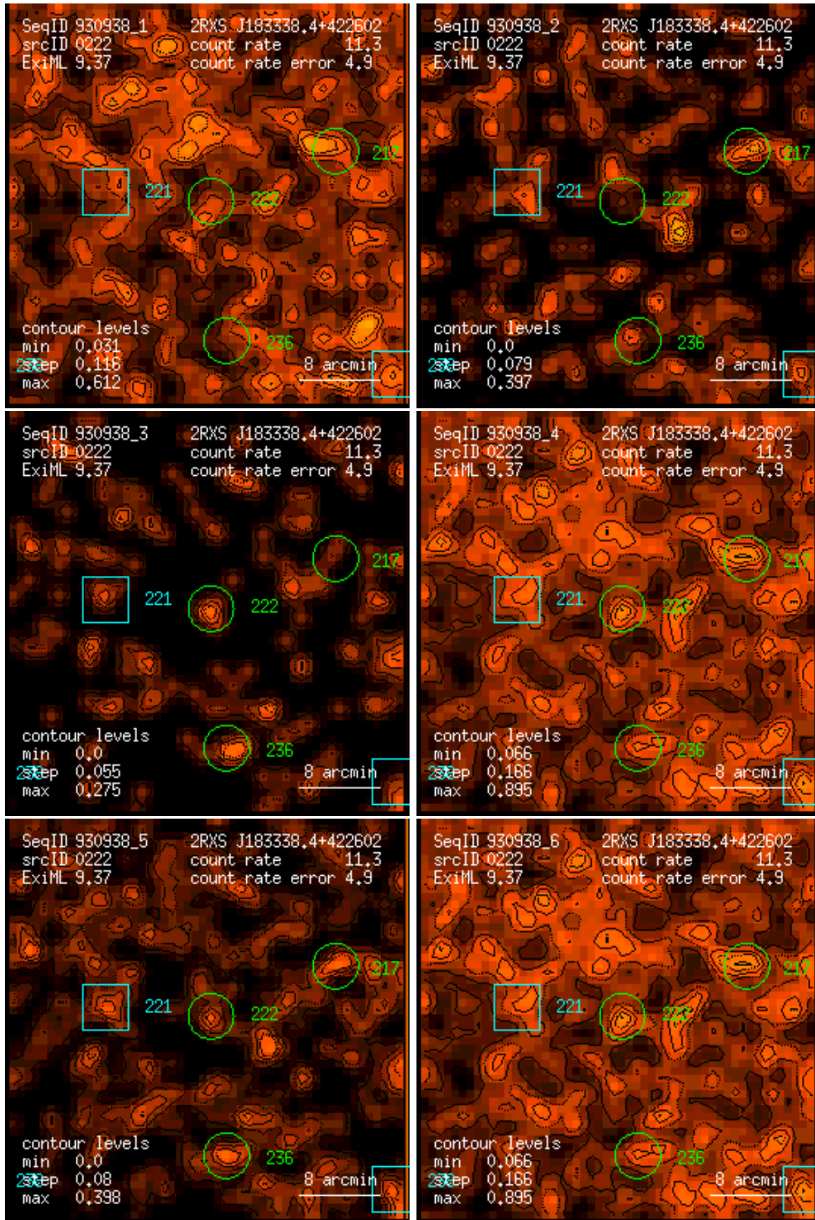
Figure 222: RASS 930938: detection 0222: band rate images, Gaussian filter: (1) PSPC channels 11 – 41, (2) 52 – 90, (3) 91 – 201, (4) 11 – 235, (5) 52 – 201, (6) 11 – 201. Broad band rates in counts/ks. Band rate contour levels in counts/ks/arcmin 2 .
